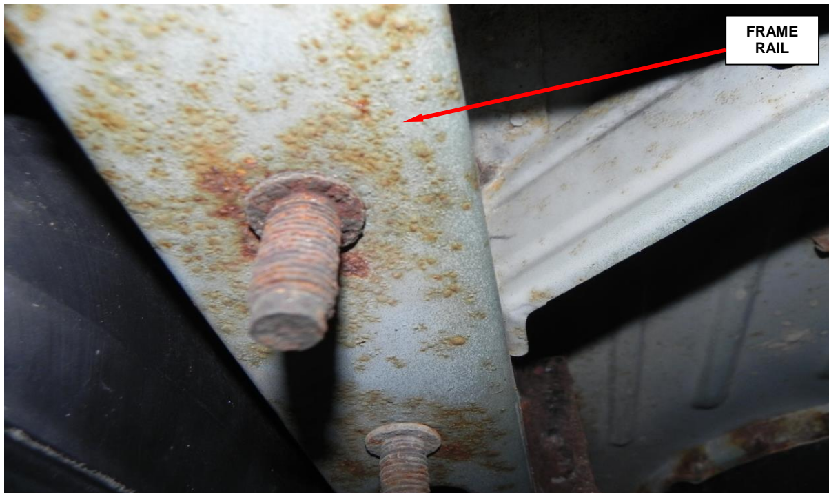
Figure 6 – Level 3 Corrosion
