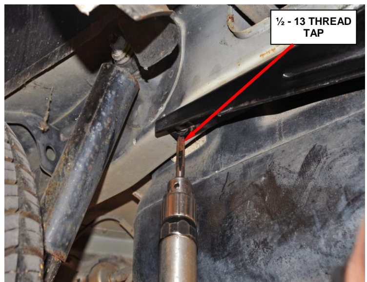
Figure 11 – Trailer Hitch Mounting Bolts (left side shown)
