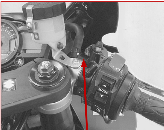
(2007 GSX-R1000 Shown) Front Brake Master Cylinder EARLY STYLE
