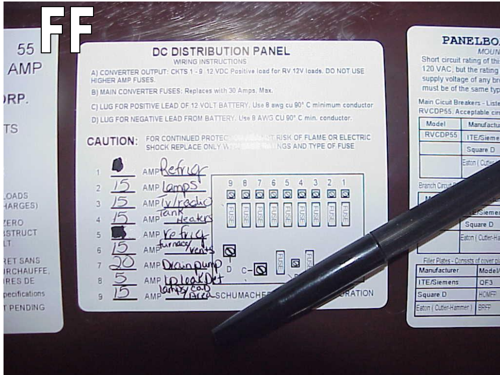
(With a Permanent Marker, Black Out the 5 and 20 Number on the Refrigerator Circuits)
