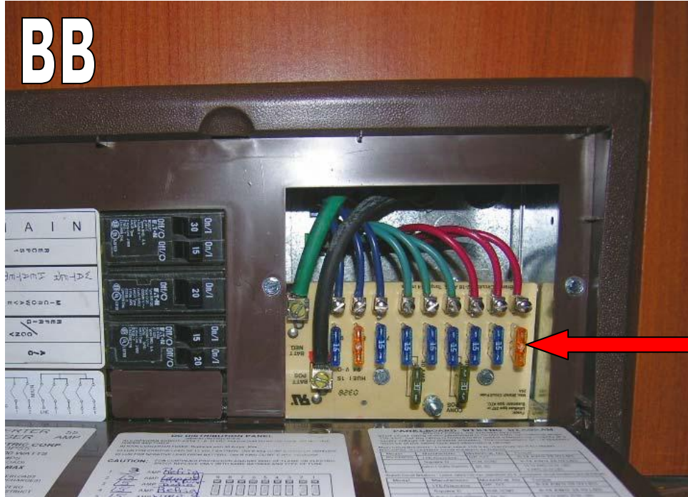
(Typical View) (Fuse Configuration May Vary By Model According to Available Equipment)
