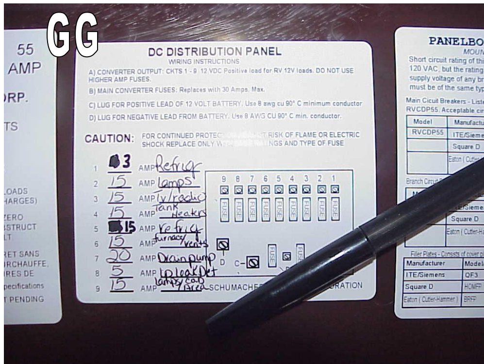
(With a Permanent Marker, Write in the "3" and "15")
