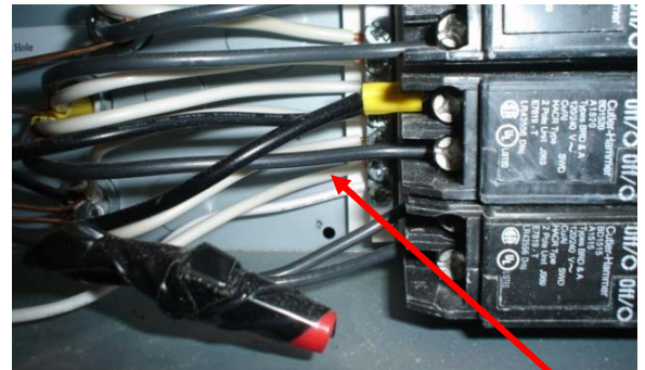
Fig. 3—Neutral wire connected to neutral bar. CORRECT
