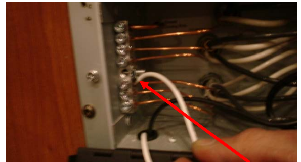
Fig. 2—Neutral wire connected to ground bar. INCORRECT
