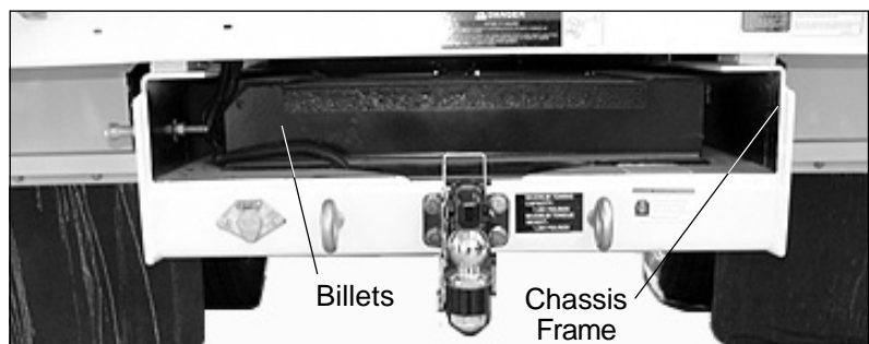
Figure 1— Counterweight Placement
