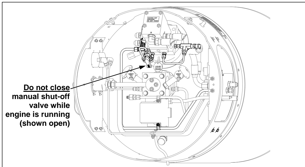
Figure 1: Manual shut-off valve must remain open
