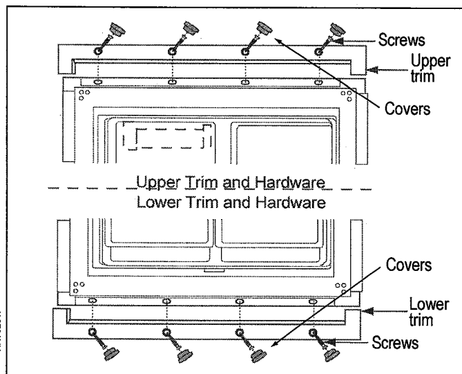
Figure 2. Removing the Upper and Lower Trim Pieces
