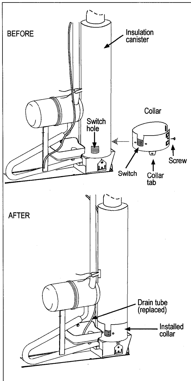
Figure 5. Installing the Metal Collar and Switch
