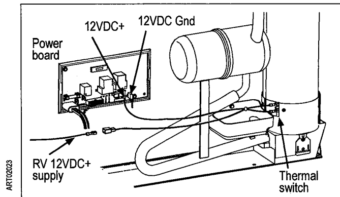
Figure 6. Connecting the Switch Electrically
