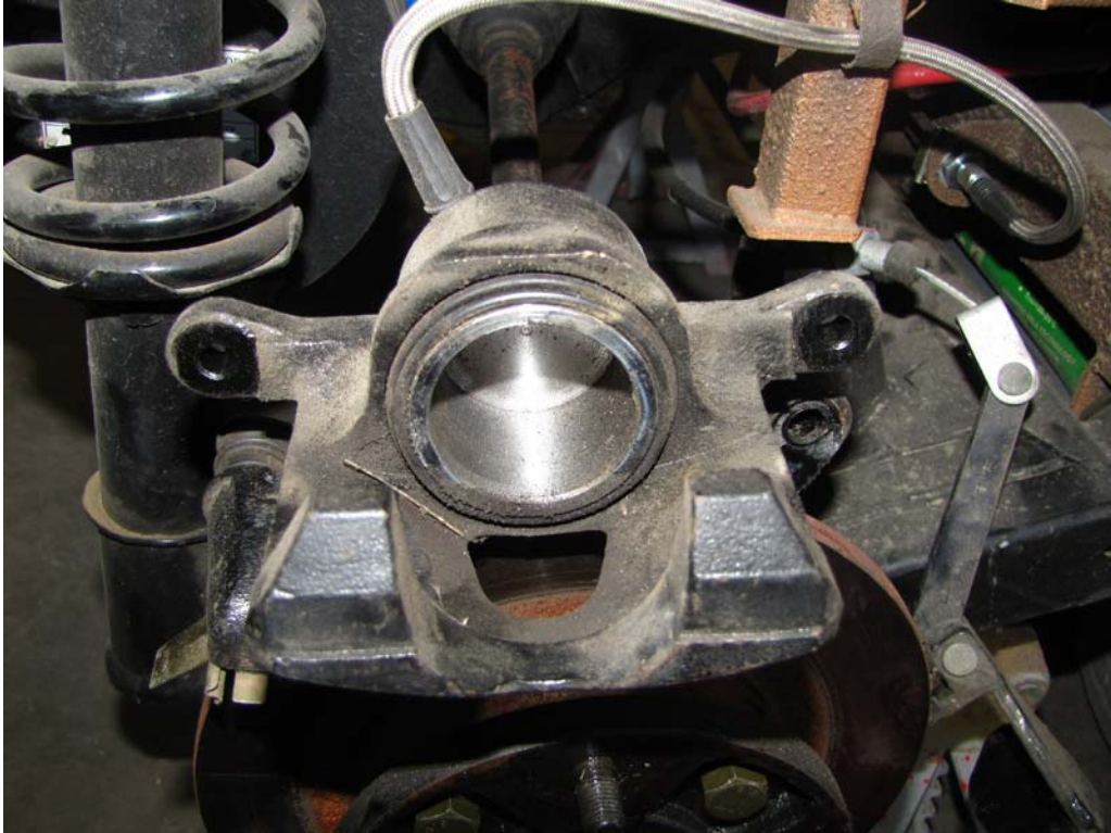
FIGURE 21. RIGHT REAR BRAKE CALIPERS AND PISTON
