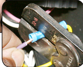
Typical Wire Splicing
