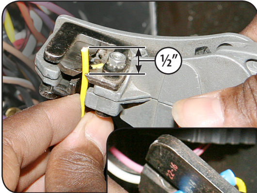
Typical Wire Stripping
