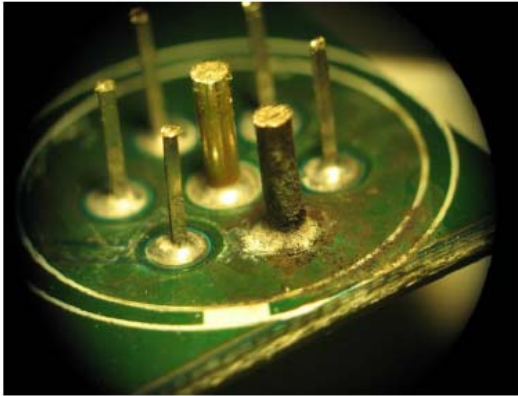
Corrosion starting on battery voltage pin
