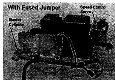
View of the fused wiring harness installed.
