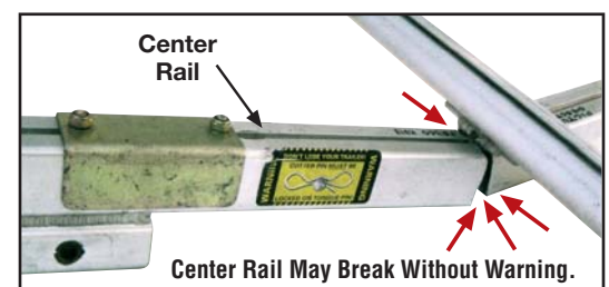
Fig. C - Broken Center Rail (simulation)
