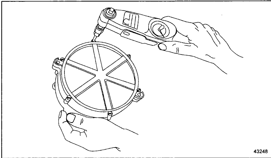
Figure 4 Torque Cover Screws to Specification
