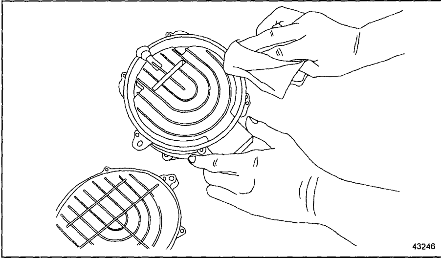
Figure 2 Clean Regulator Cover and Body Mating Surfaces
