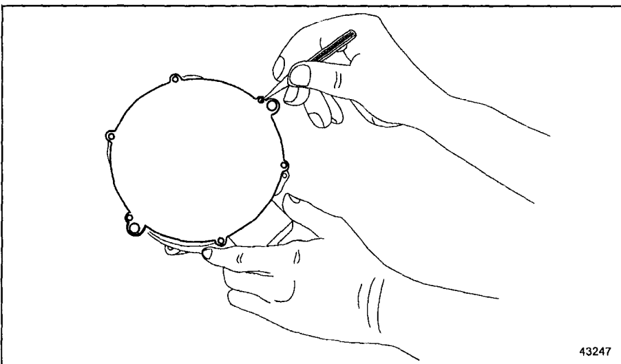
Figure 3 Align Gasket Index Holes with Regulator Body
