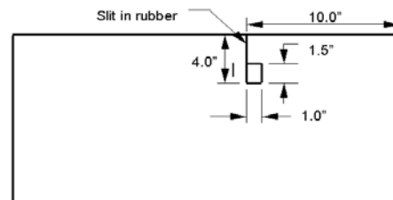
Template for splash shield
