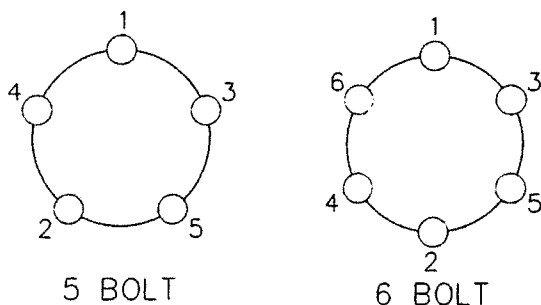
Pattern for tightening lug nuts
