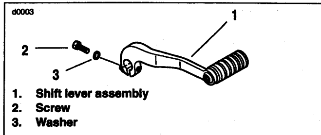
Figure 5. Shift Lever
