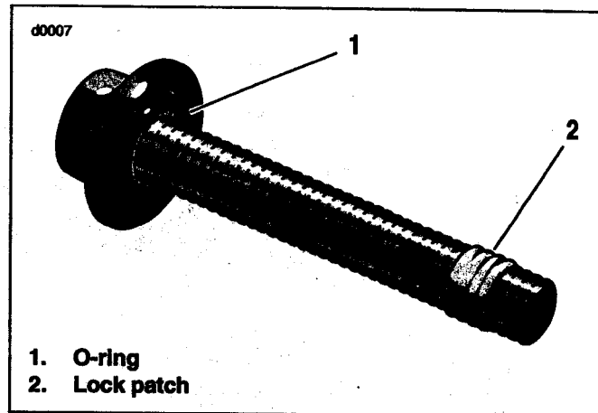
Figure 17. Sealing Fastener (Part No. 786A)
