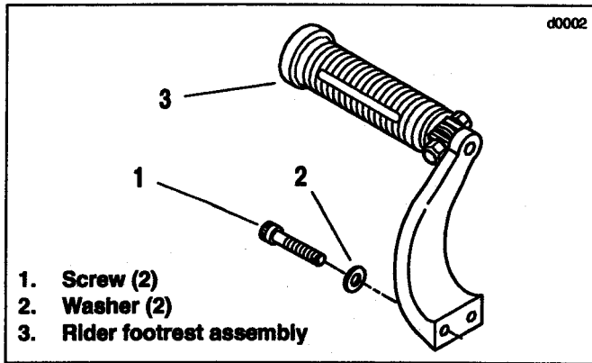
Figure 4. Left Rider Footrest Assembly
