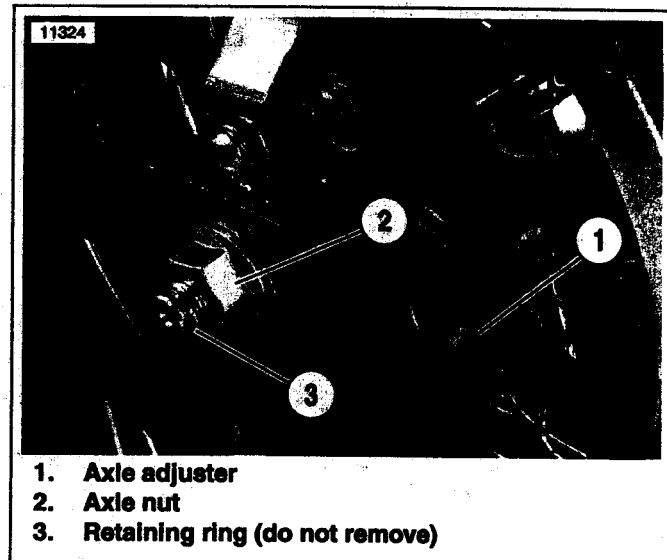
Figure 3. Axle Adjusters
