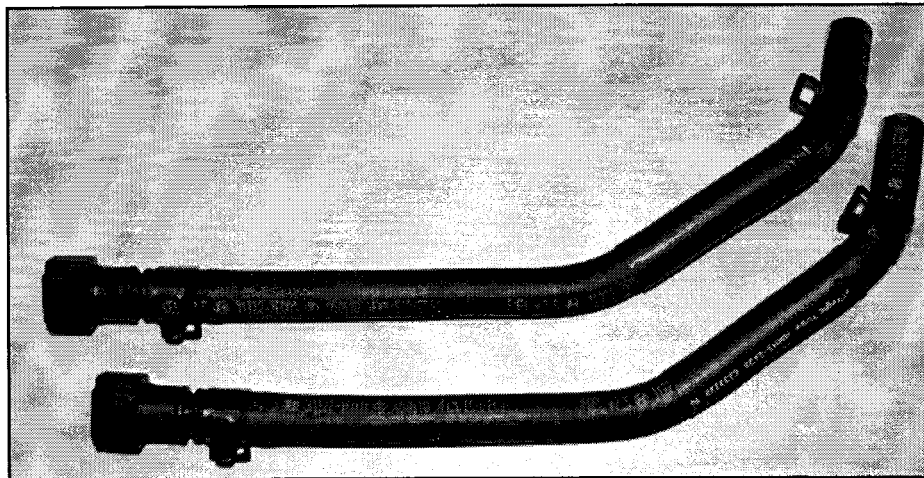
Fuel Hose — (P/N: Q3132 23E000Q Consists of One [1] Fuel Hose) - Two (2) Required Per Vehicle
