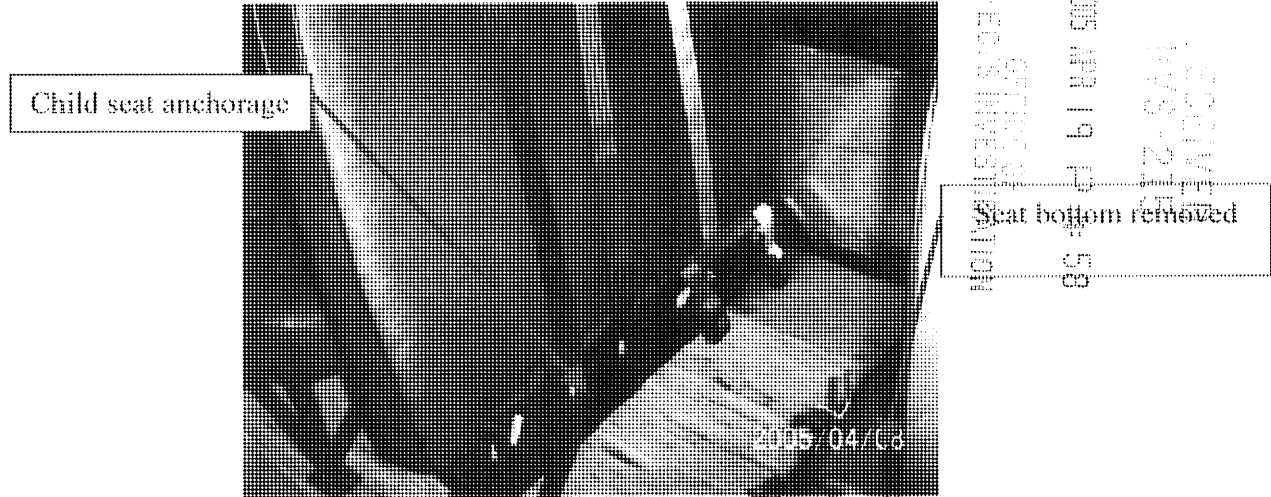
Picture 1: Seat without seat bottom
