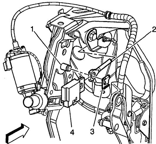
Adjustable Brake Pedal Pushrod Retaining Clip (3)
