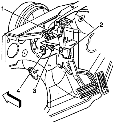
Non Adjustable Brake Pedal Pushrod Retaining Clip (4)
