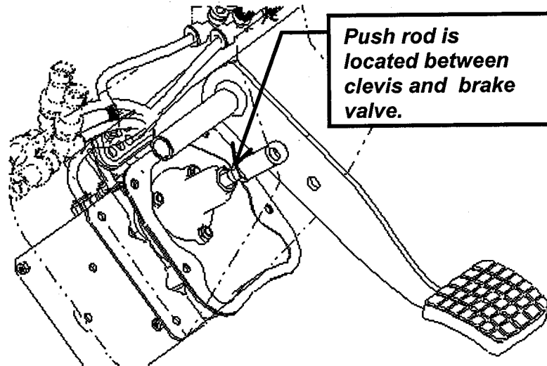
Figure – Push Rod Location
