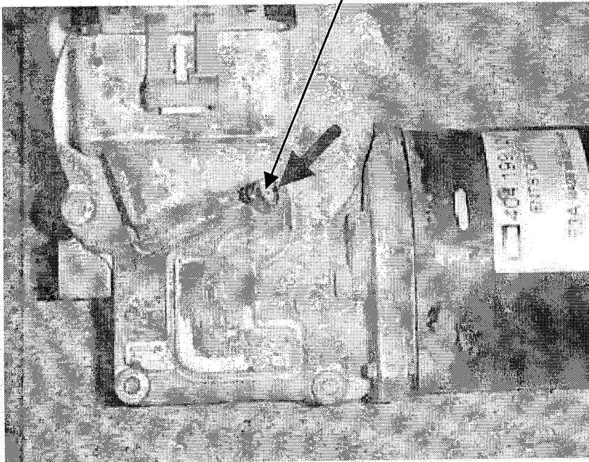
Example of melted connector (plastic deformed)
