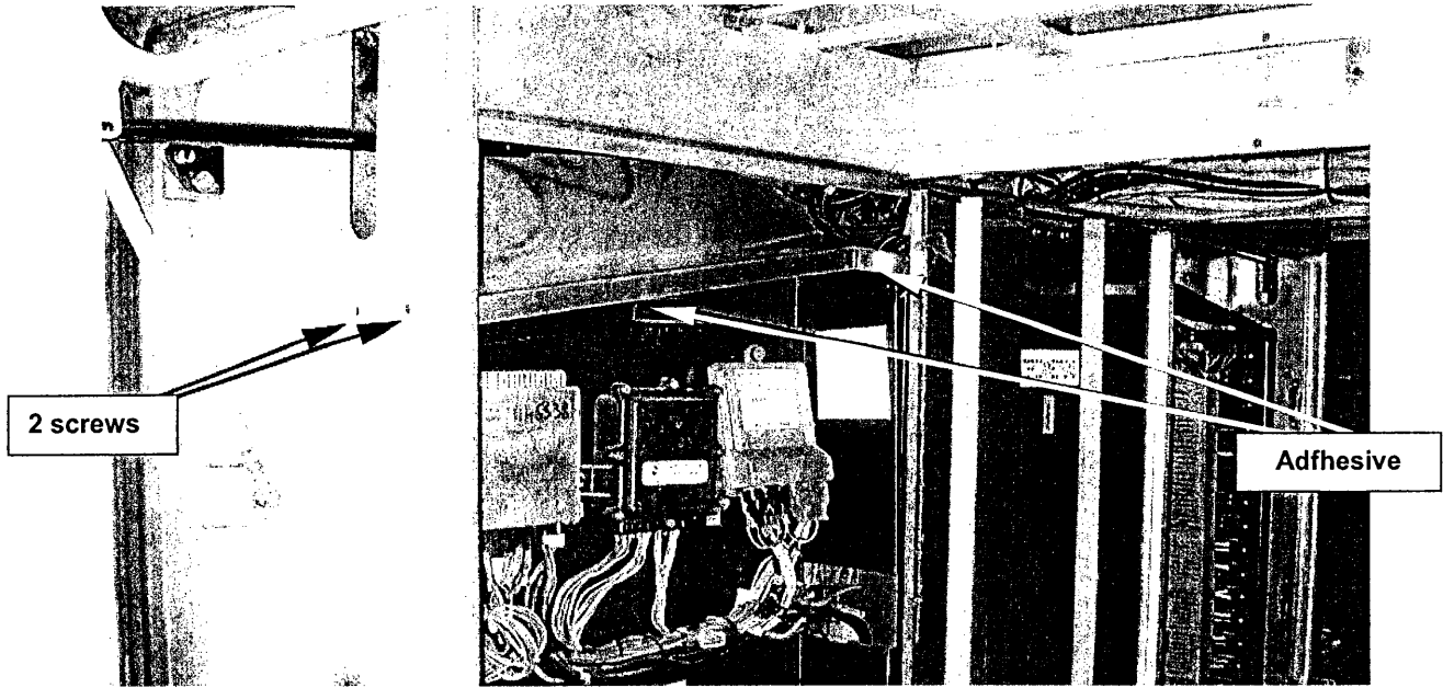
Figure 2: VH 10906063 – new part installation
