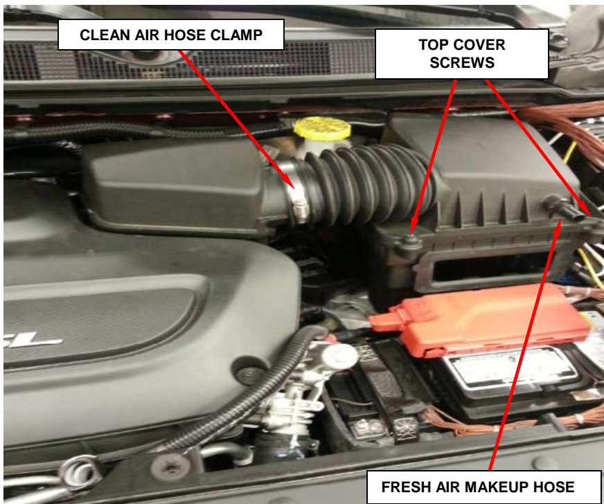
Figure 27 – Air Cleaner Housing
