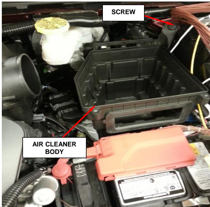
Figure 28 – Air Cleaner
