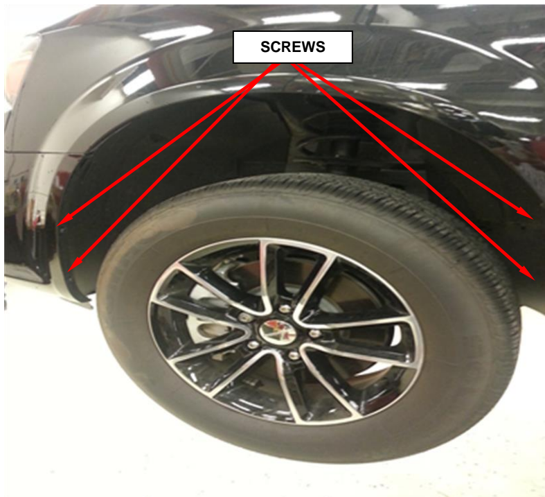
Figure 21 – Right Front Splash Shield
