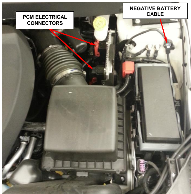
Figure 23 – Negative Batter Cable
