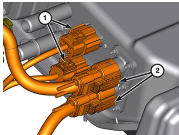
Figure 17 – Wire Harness
