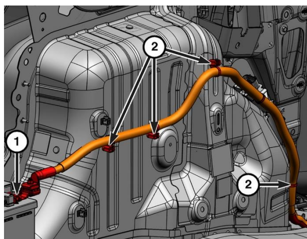
Figure 46 – 12-Volt Cable
