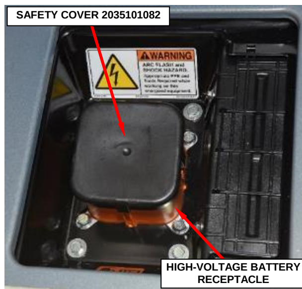
Figure 13 – High-Voltage Battery Receptacle Safety Cover
