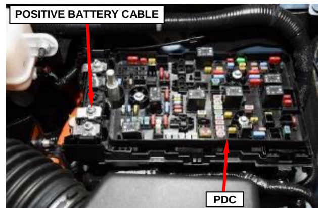
Figure 6 – Positive Battery Cable
