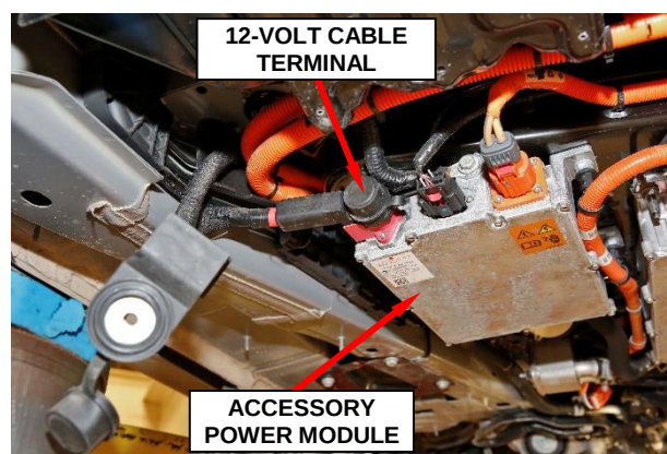
Figure 37 – 12-Volt Cable
