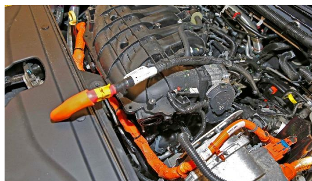
Figure 30 – 12-Volt Cable
