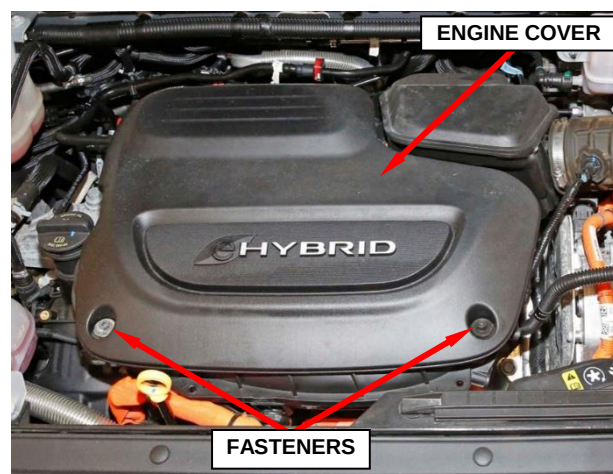
Figure 26 – Engine Cover
