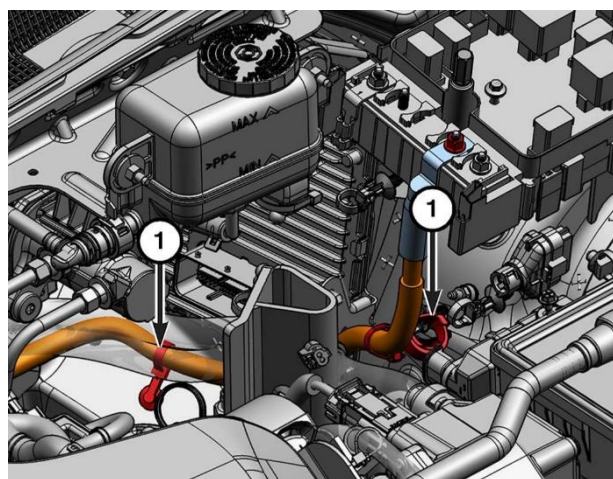
Figure 28 – 12-Volt Cable Clips
