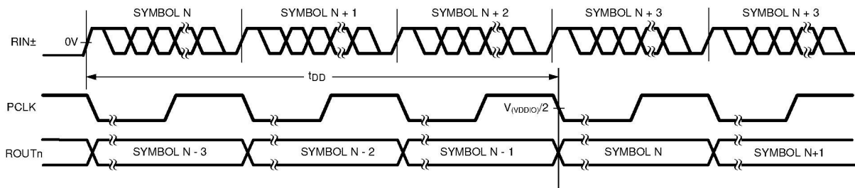
Figure 4-6. Deserializer Delay
