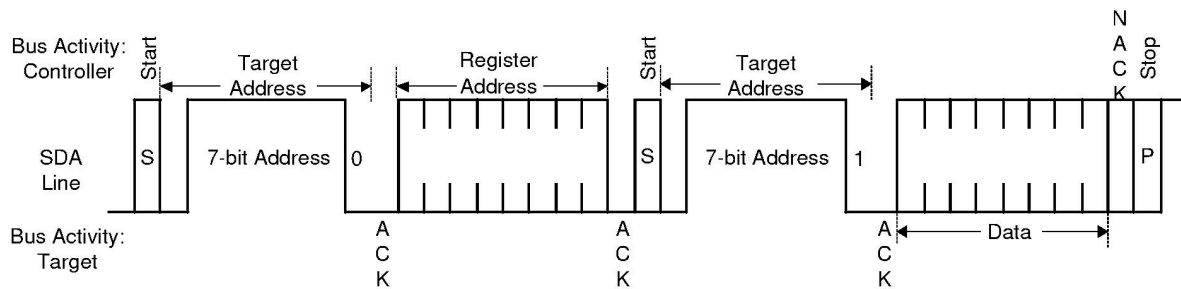
Figure 5-8. Serial Control Bus — READ
