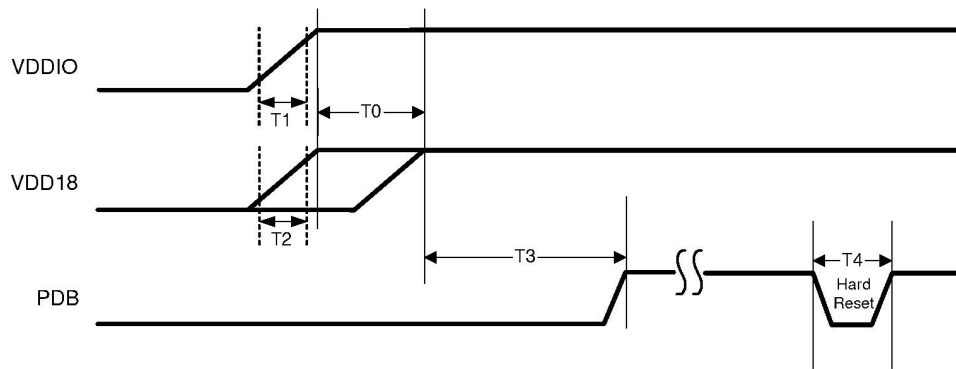
Figure 6-11. Power-Up Sequencing
