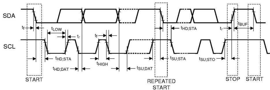
Figure 5-10. Basic Operation
