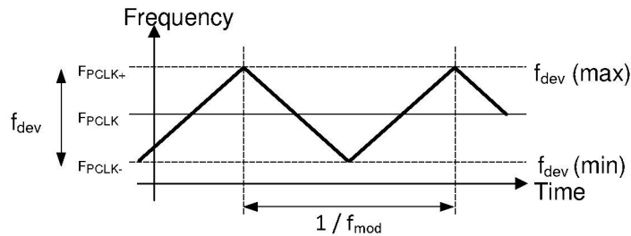
Figure 4-9. Spread Spectrum Clock Output Profile
