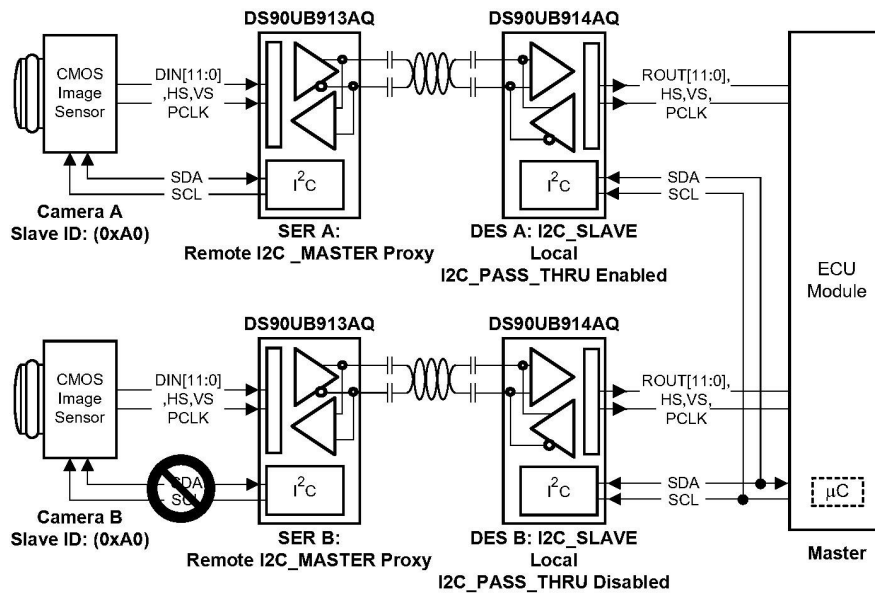
Figure 25. I2C Pass-Through
