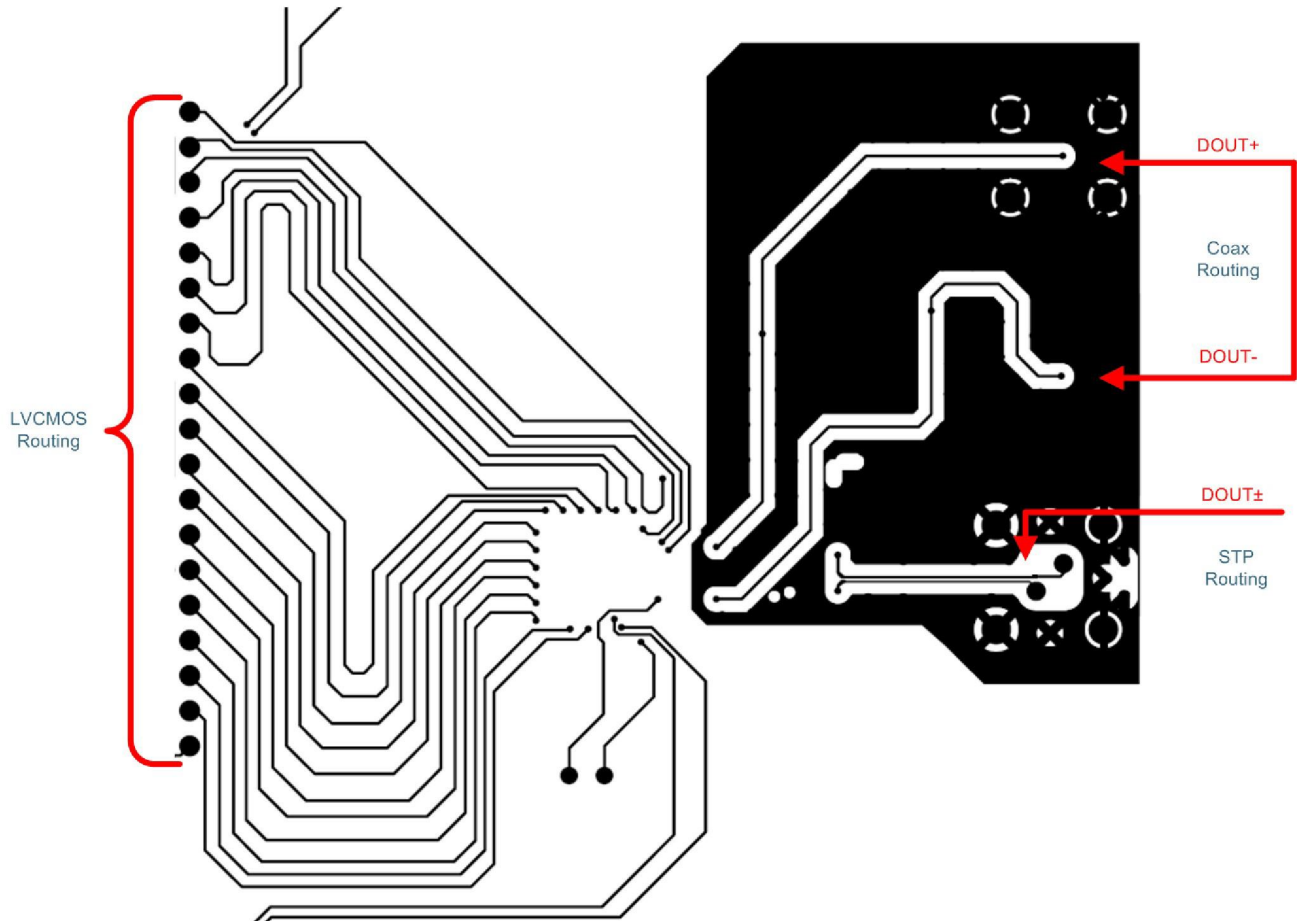
Figure 40. DS90UB913A-Q1 Serializer Example Layout
