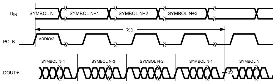
Figure 10. Serializer Delay
