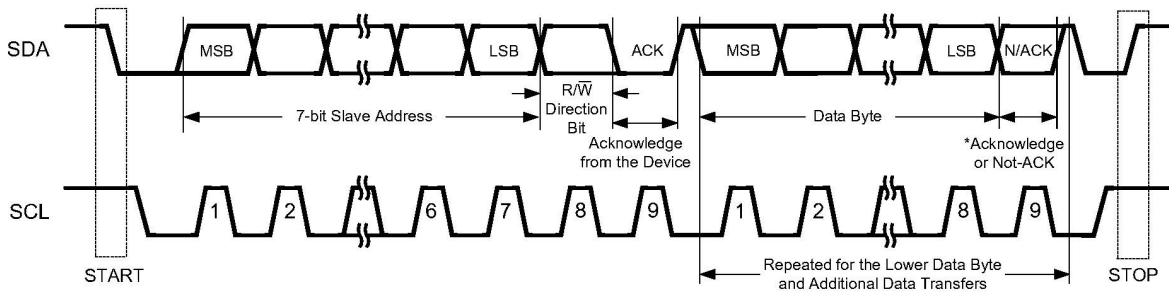
Figure 23. Basic Operation
