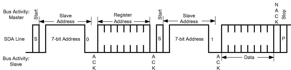
Figure 22. Read Byte
