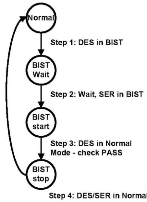
Figure 19. AT-Speed BIST System Flow Diagram
