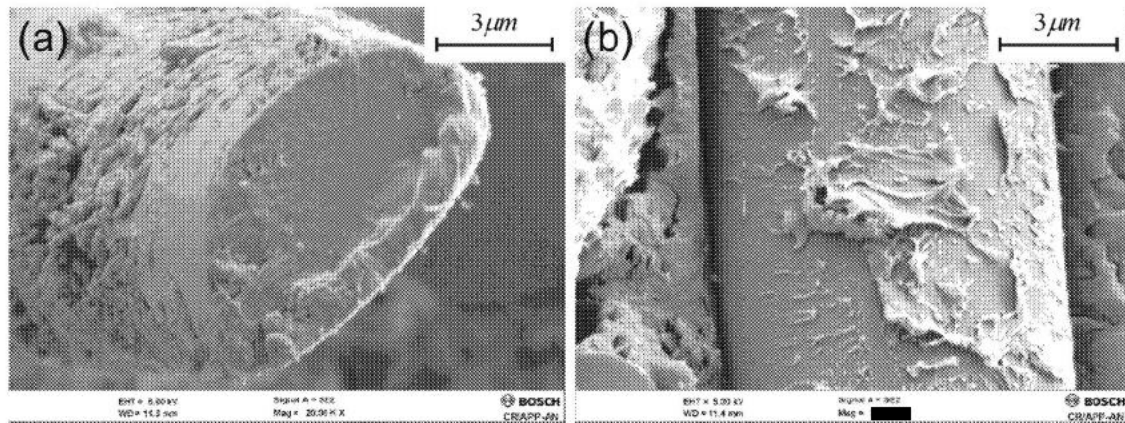
Figure 12. Fiber-matrix adhesion on the fracture surface of a notched specimen caused by stable FCP; (a) Fiber perpendicular to the fracture surface; (b) Fiber lying on the fracture surface.
