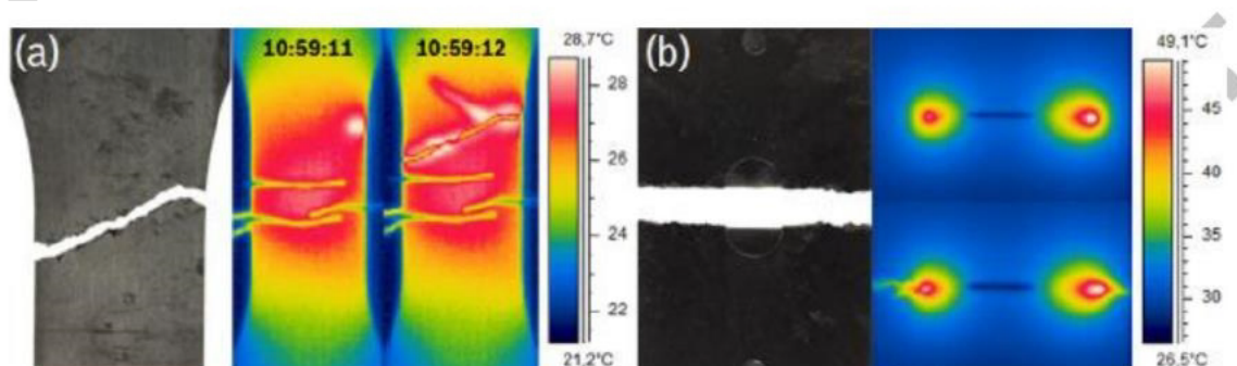
Figure 3. Crack path and temperature distribution at failure in (a) Plain specimens; (b) Notched specimens.
