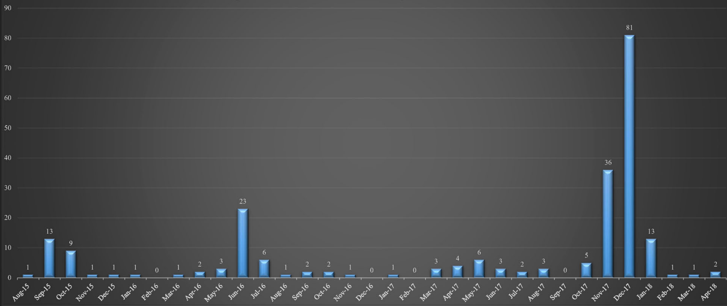
1.0L Fox Classic Oil Pump Belt Tensioner Failures by Vehicle Production Month
