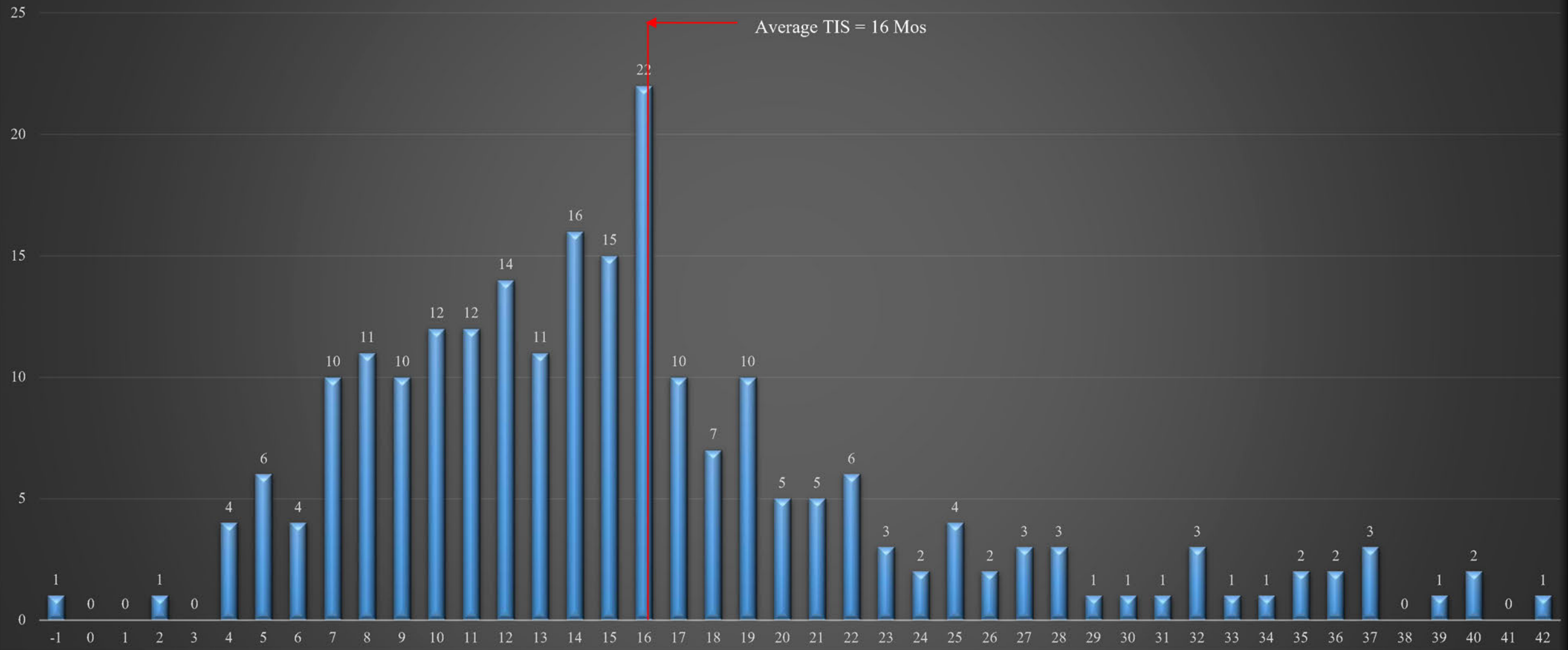
1.0L Fox Classic Oil Pump Belt Tensioner Failures by TIS
