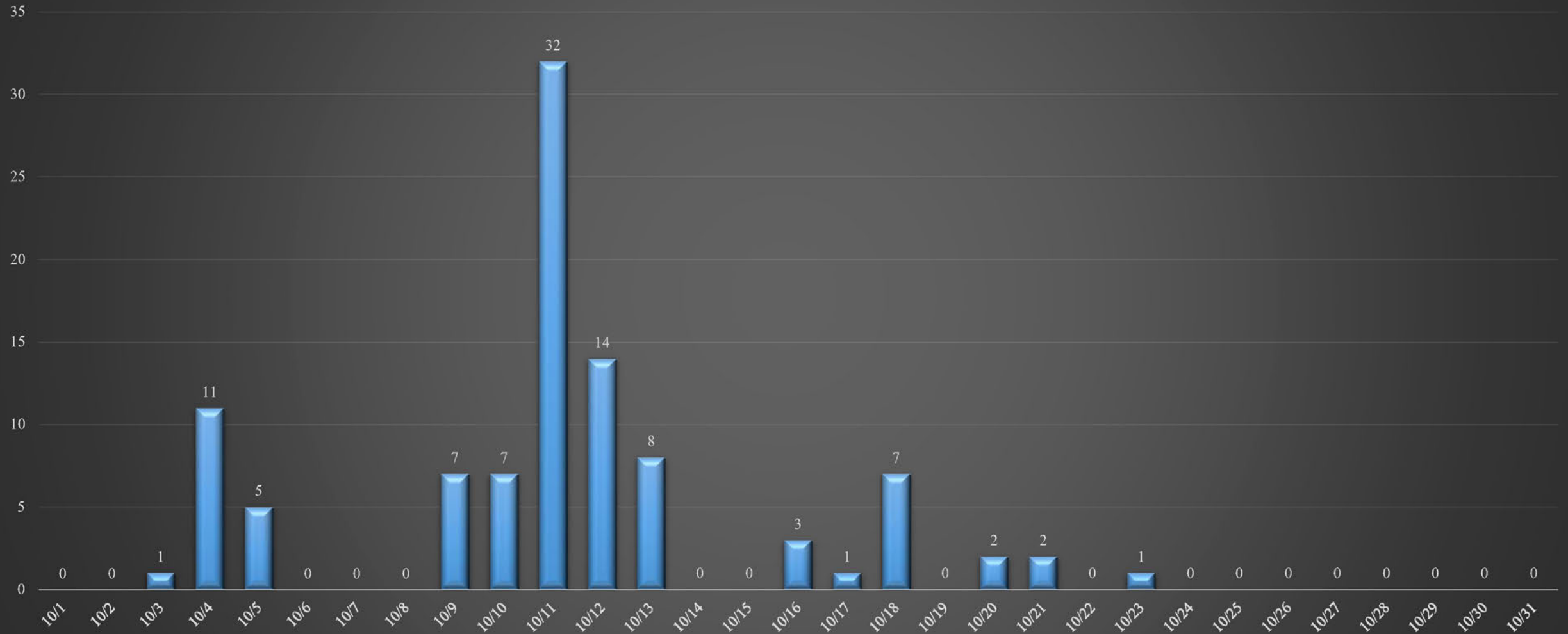
1.0L Fox Classic Oil Pump Belt Tensioner Failures by Engine Production Date - Oct. 2017
