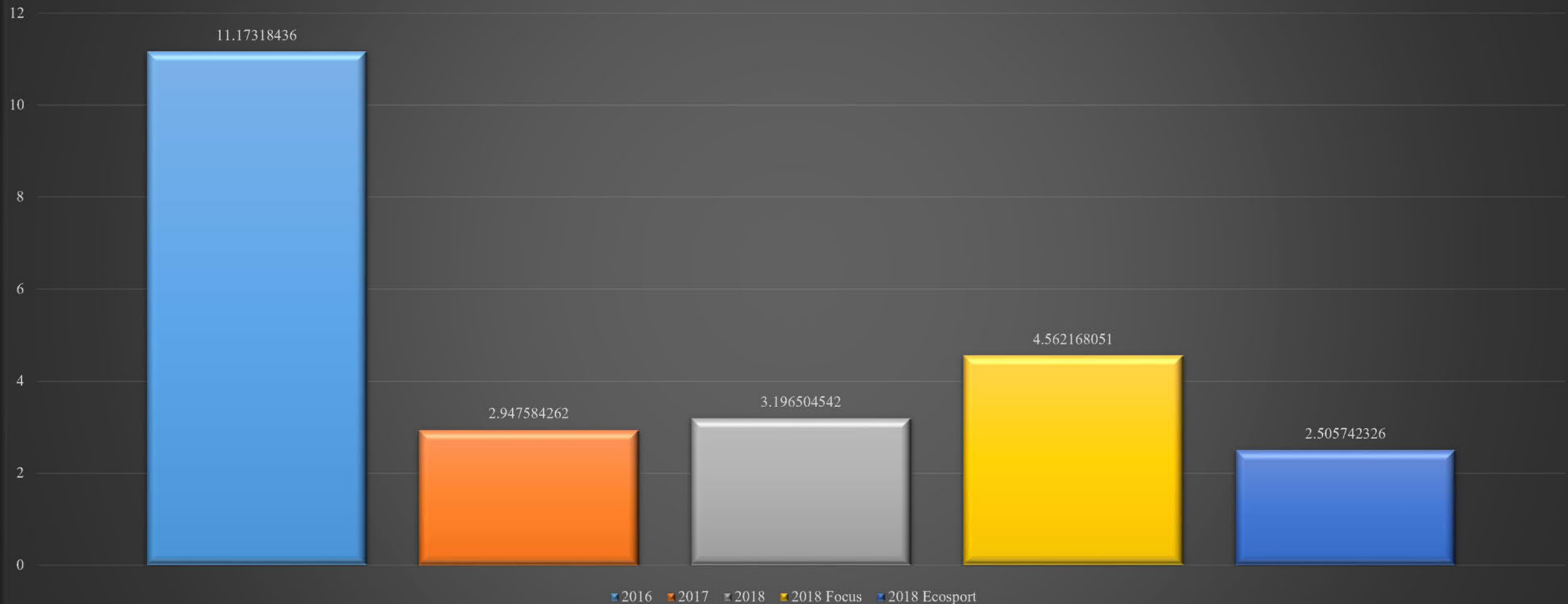
R/1000 for Vehicles Produced - 2016,2017,2018MY 1.0L Fox Classic Oil Pump Belt Tensioner Failure
