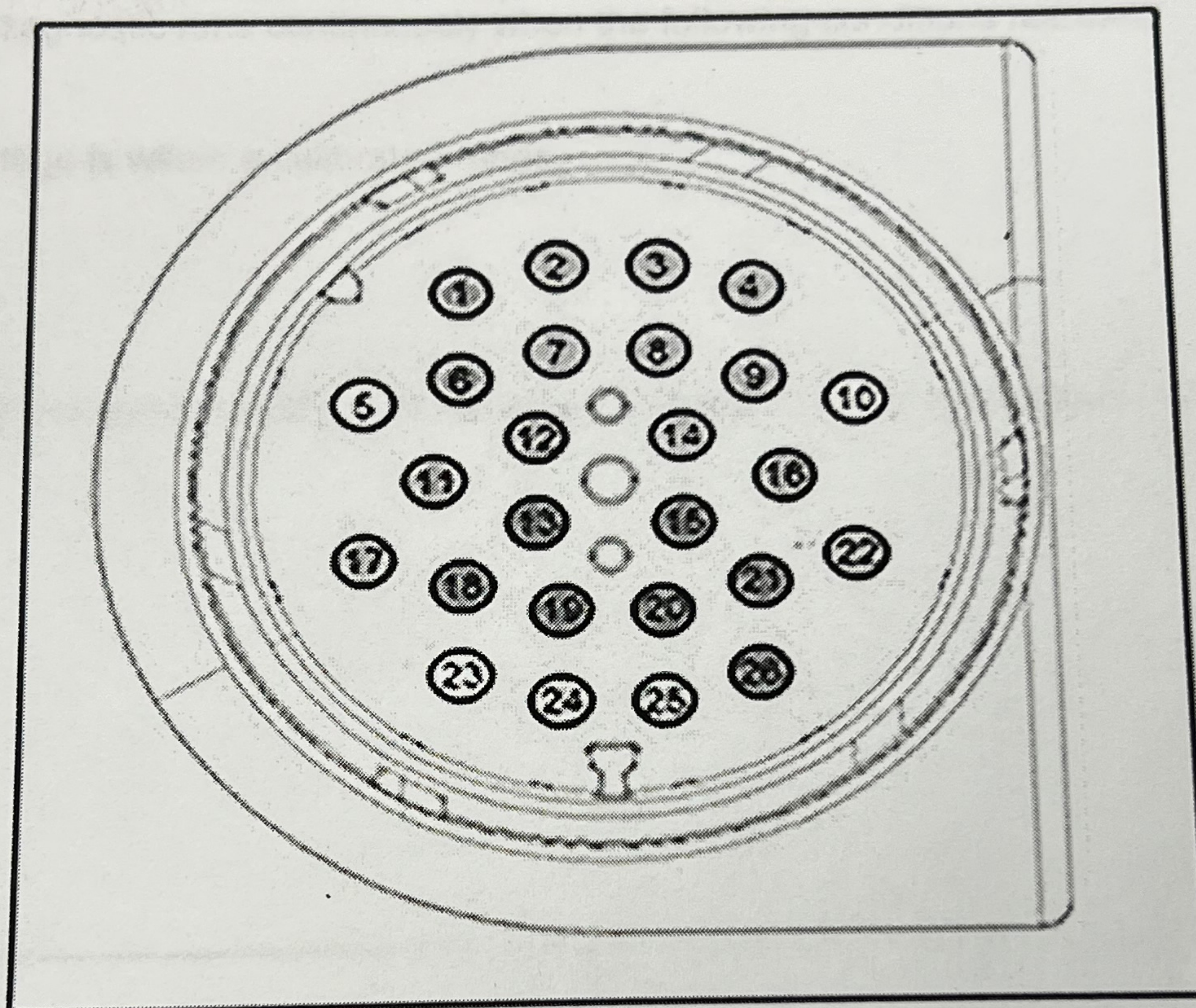
Pinout view of 26 Pin Trans Connector
