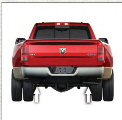
Rear Jacking Locations
