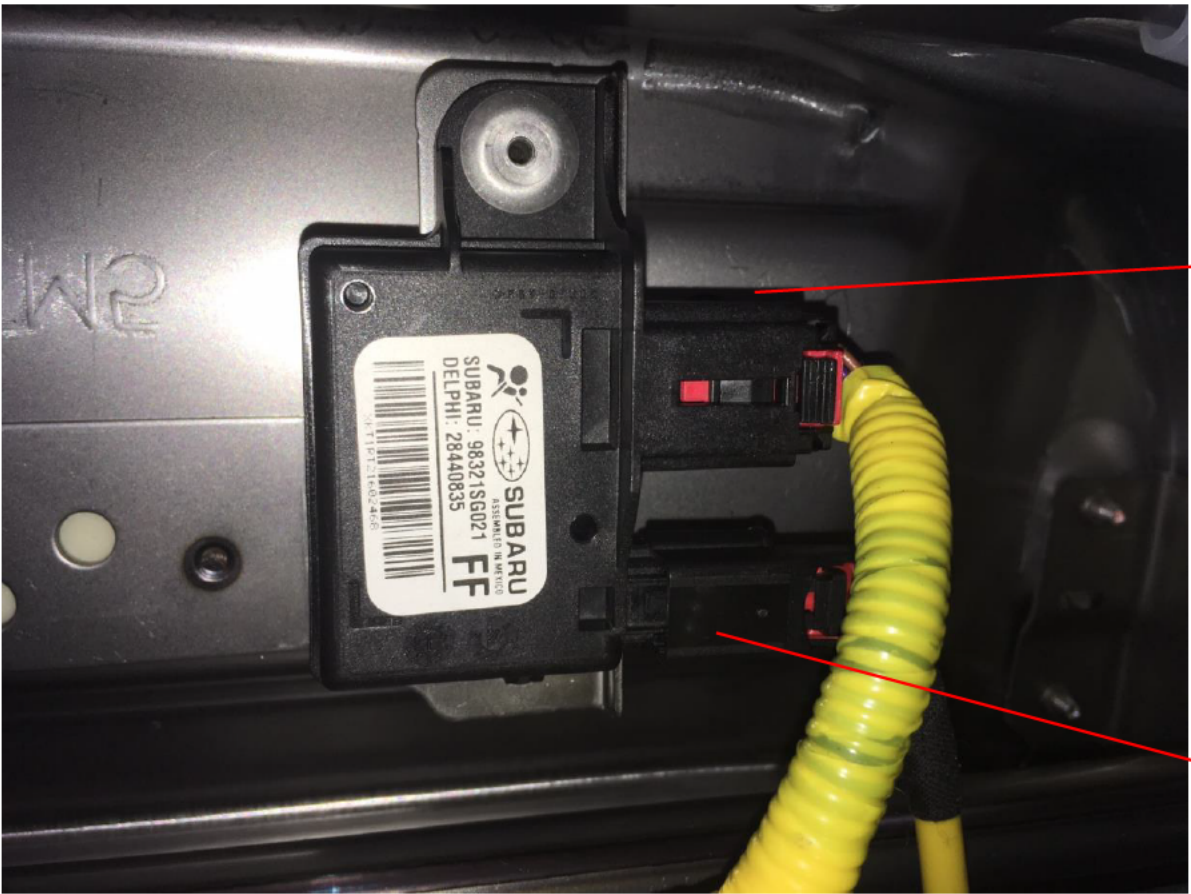
ODS Control Module Connectors Fully Seated and Locked-No Loose or Bent Terminals
