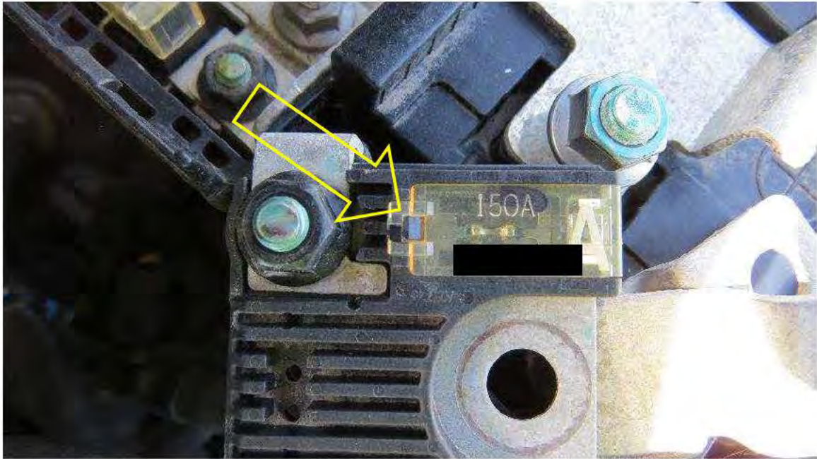
Photograph 7: No damage to the 150-amp fuse for the alternator cable.
