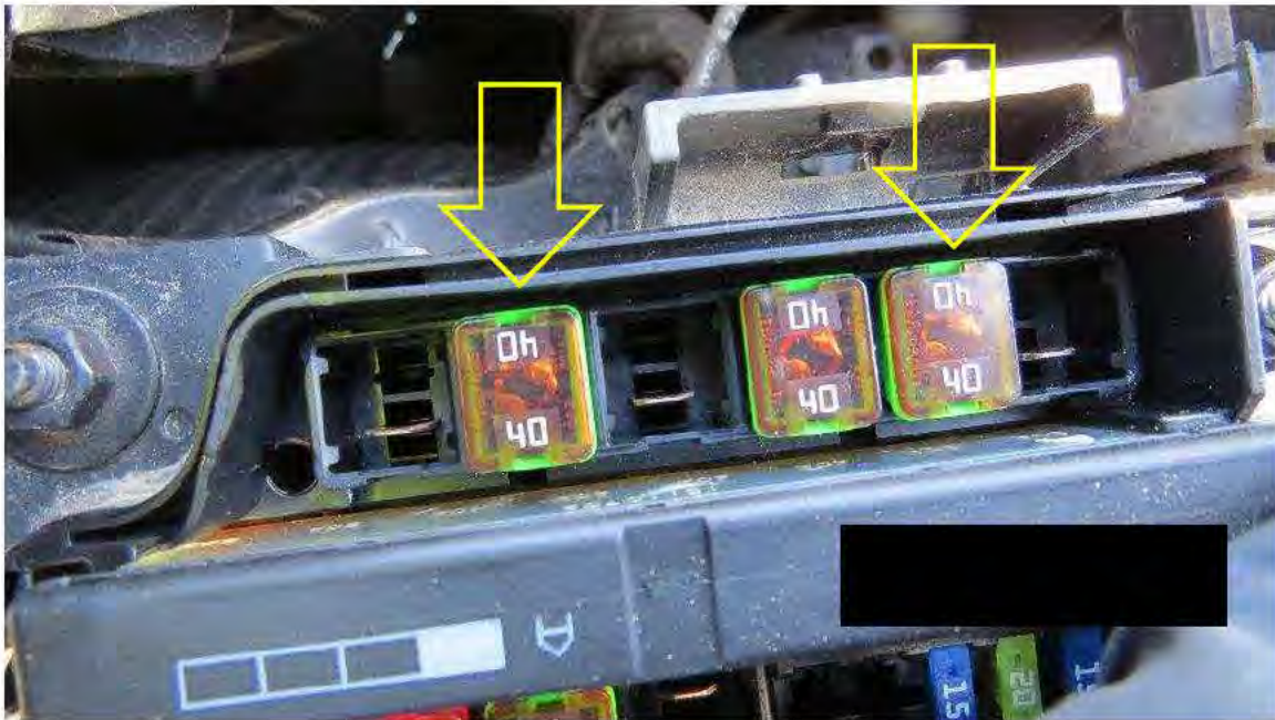
Photograph 9: 40-amp fuses identified as IG1 and IG2 have activated (blown).
