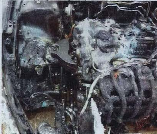
22. View of the passenger's side engine compartment from the front.
