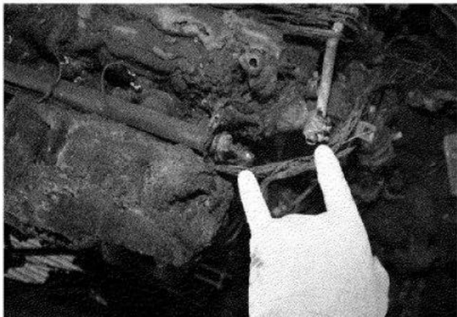
Photo No. 10: View of fuel rail end & end of metal fuel line
