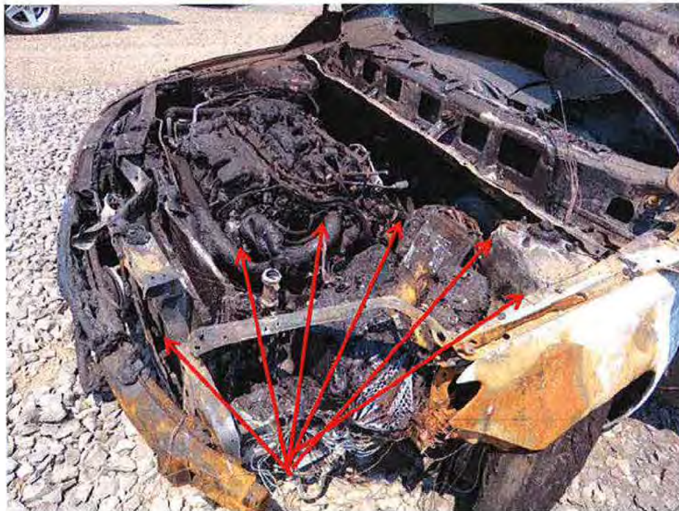
22 The red arrow's depict the direction of fire travel from the head light area of the vehicle into the interior of the engine compartment
