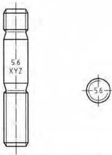
Figure 14 — Example of marking of studs
