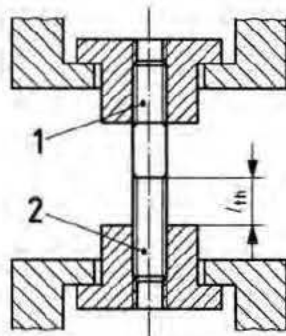
c) Example of testing device for studs
