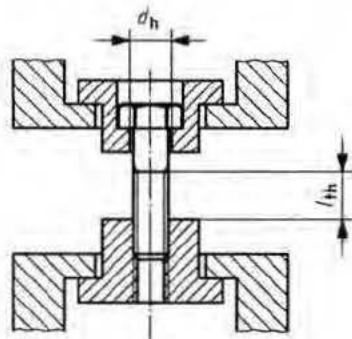
a) Example of testing device for bolts
