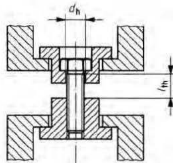
b) Example of testing device for screws
