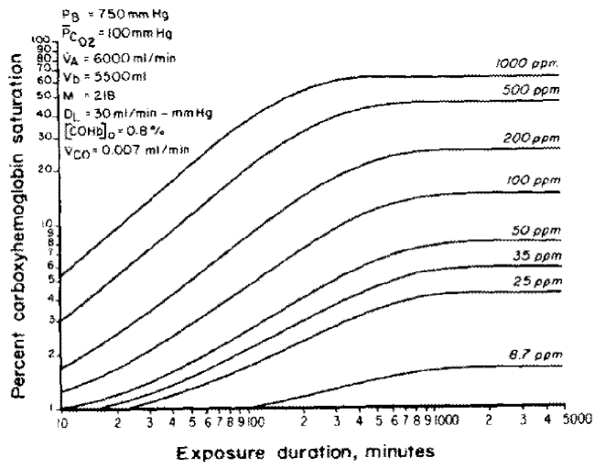
FIGURE 2-2 COHb for different exposure concentration-time combinations. Source: Peterson and Stewart 1975.
