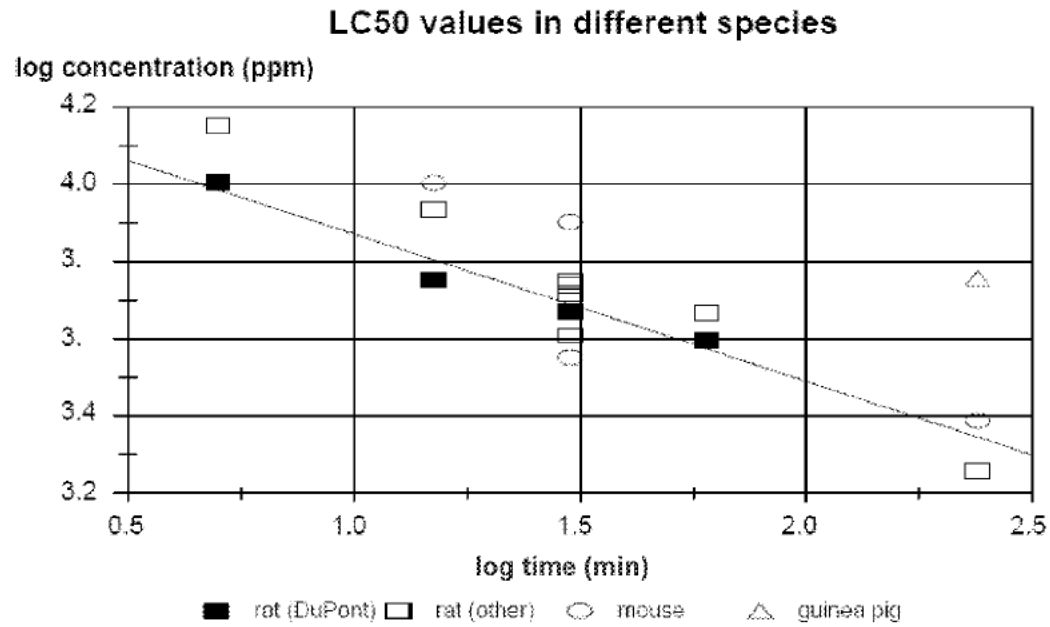
FIGURE 2-1 LC 50 values for CO in different species.
