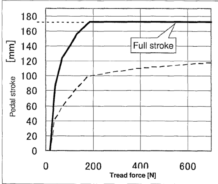
Value of a pedal ratio of 3.6 (GVW \geq 8 t)
