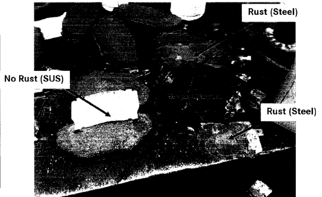
Fig2. Brake shim photo of VIN: JL6CRE1A7CK000374
