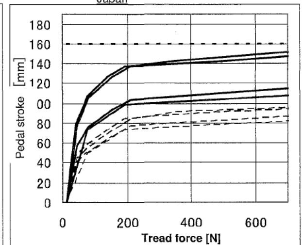
DISC vehicle for Japan
