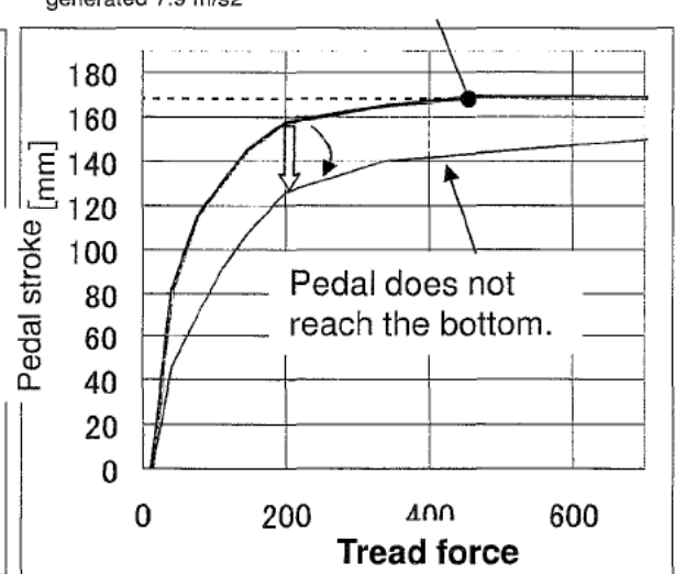
TD Φ252 vacuum servo vehicle
