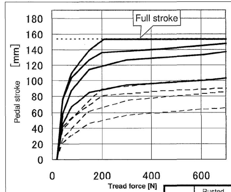
Value of a pedal ratio of 3.2 (GVW < 8 t)
