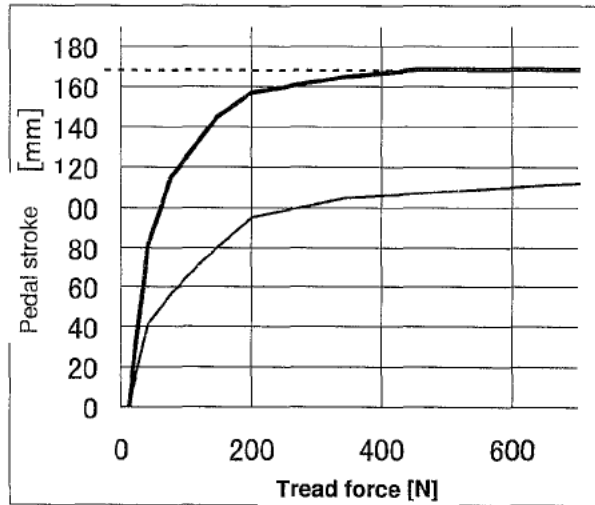
\Phi 252 vacuum servo vehicle
