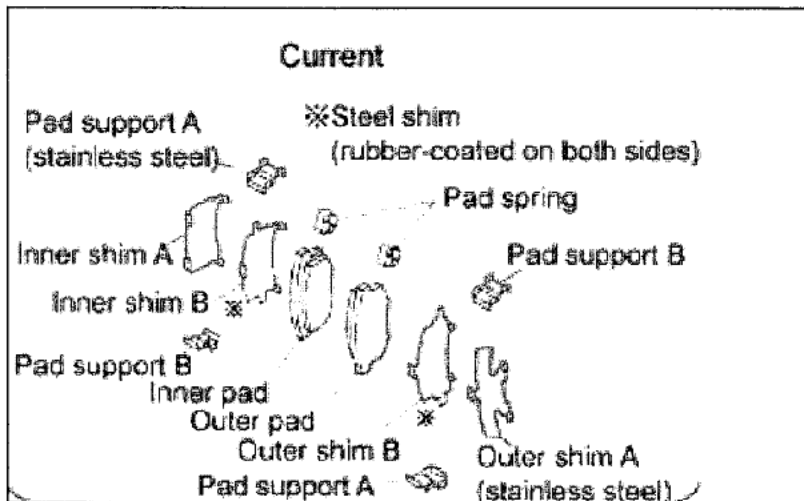
Fig 01. Composition of Brake pad
