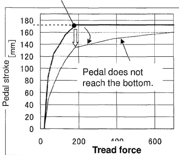
LIFT Φ252, pedal ratio 3.6 vehicle (GVW ≥ 8 t)
