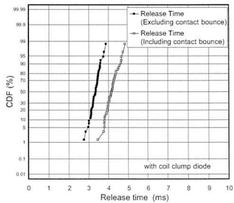
Release Time
