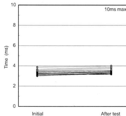
Release time
