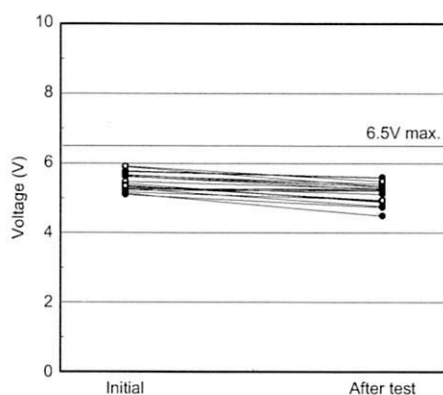
Operate voltage
