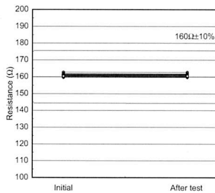
Coil resistance
