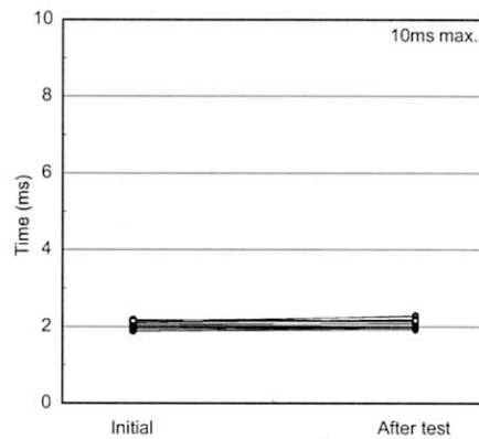
Operate time
