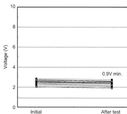
Release voltage
