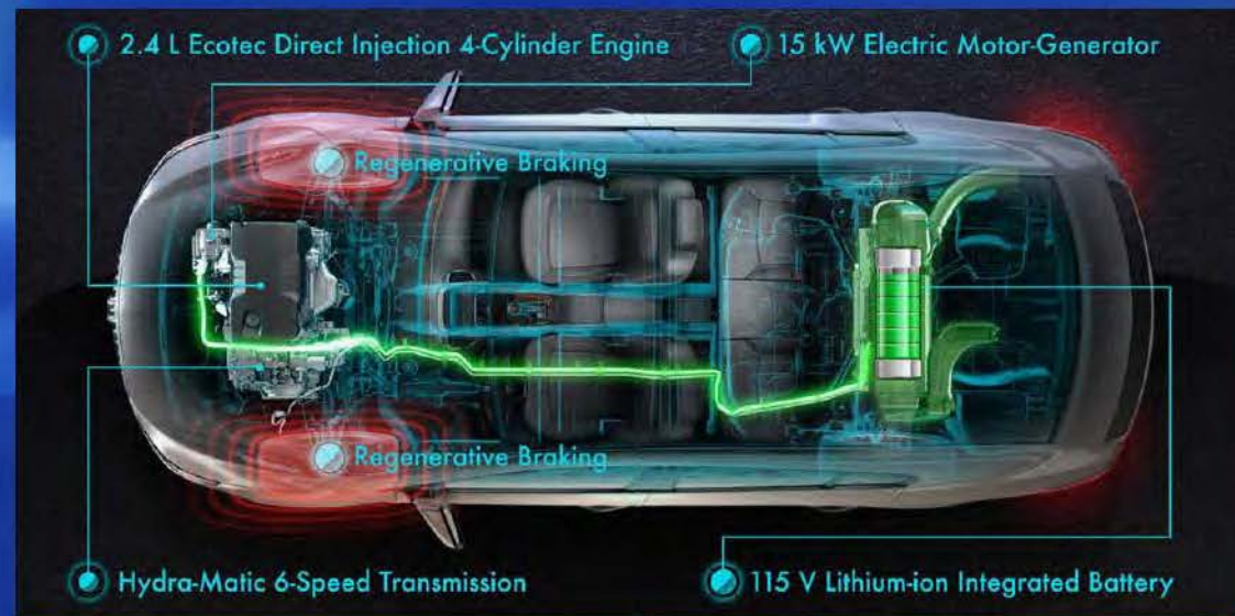
2012 LaCrosse 2.4L Ecotec with eAssist™ Technology
