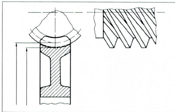
Fig. 8.13 One piece worm gear
