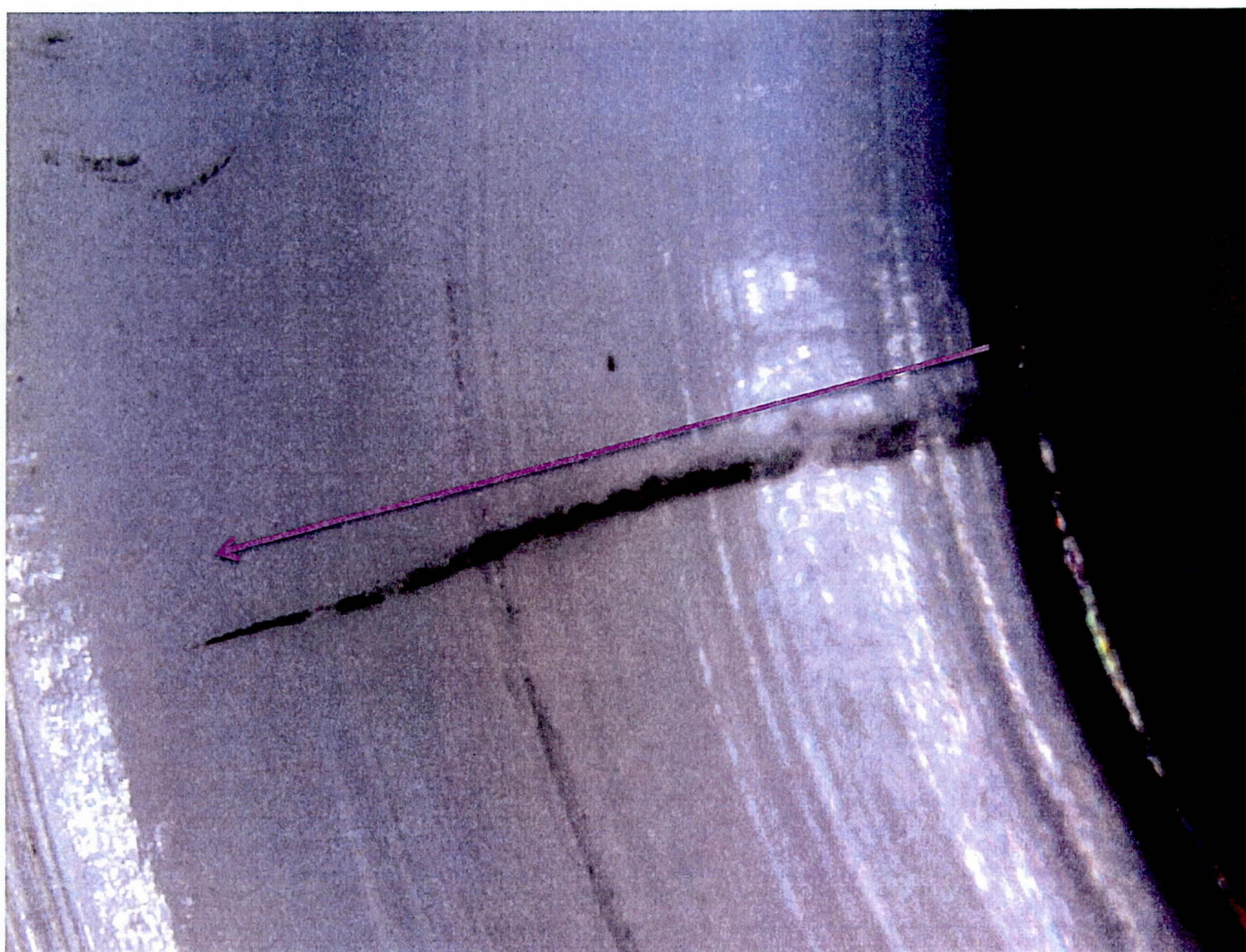
Radial fracture at insert.
