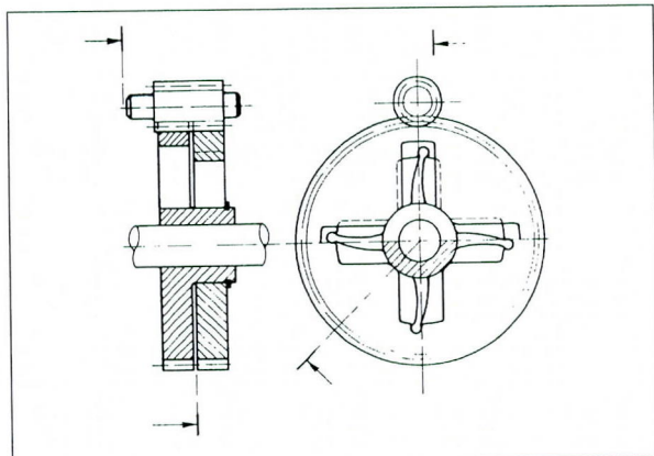
Fig. 8.23 Backlash-free gear
