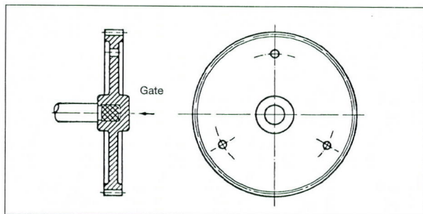
Fig. 8.09 Centre gated gear
