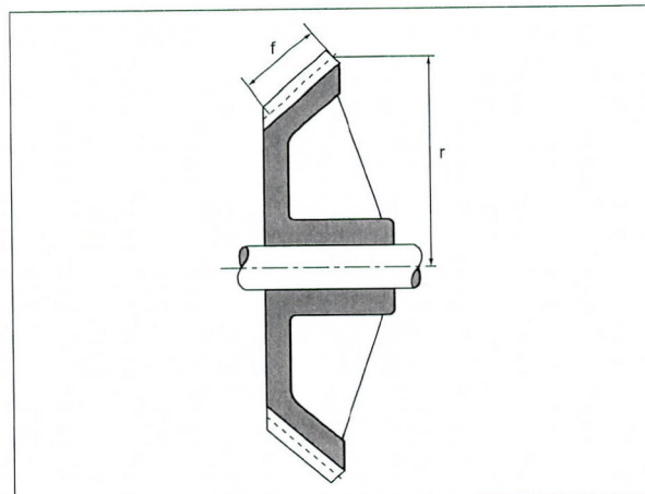
Fig. 8.06 Ribbed bevel gear
