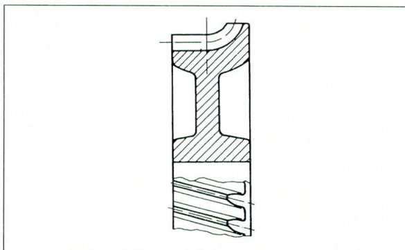
Fig. 8.15 Half throated worm gear
