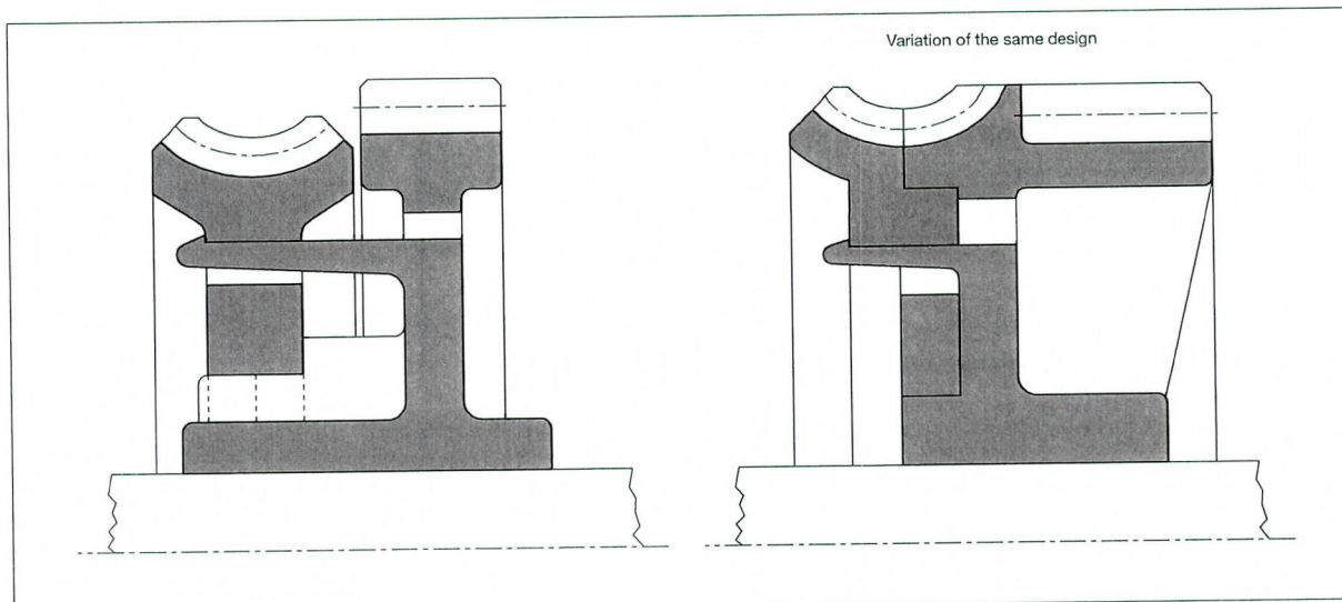
Fig. 8.17 Snap-fit split worm gear
