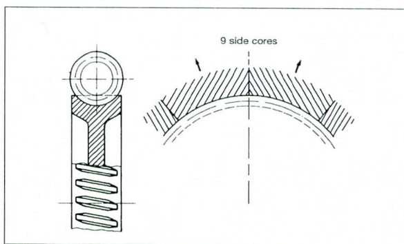
Fig. 8.14 Side-cored worm gear
