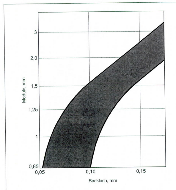
Fig. 8.12 Suggested backlash for gears of DELRIN® and ZYTEL®
