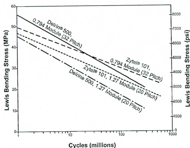
Figure 5. Maximum Bending Stress for Continuously Lubricated Gear Teeth
