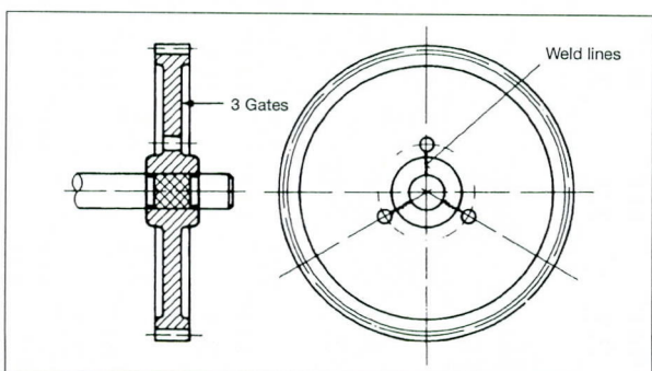
Fig. 8.10 Web gated gear
