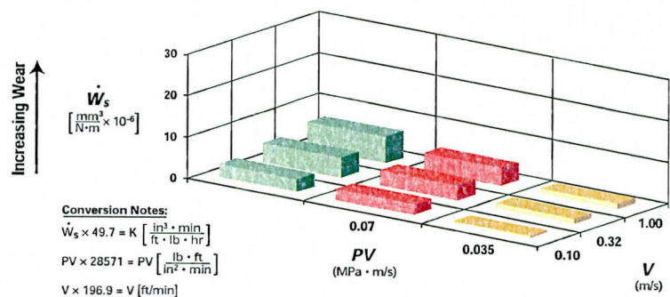
Figure 2. Delrin® 500AL Against Itself: Equilibrium-Specific Wear Rate
