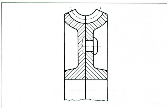
Fig. 8.16 Split worm gear
