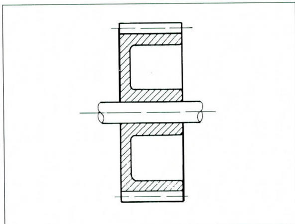
Fig. 8.04 Gear with off-centre web
