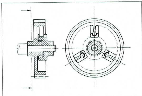
Fig. 8.24 Torque limiting gear
