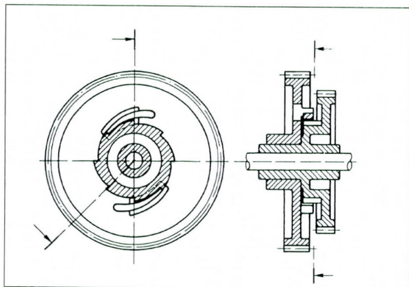
Fig. 8.20 Ratchet and gear combined
