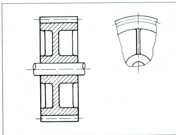
Fig. 8.05 Effect of radial ribs
