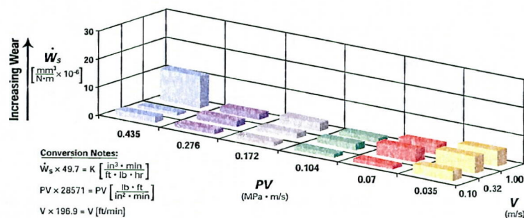
Figure 1. Delrin® 520MP Against Steel: Equilibrium-Specific Wear Rate
