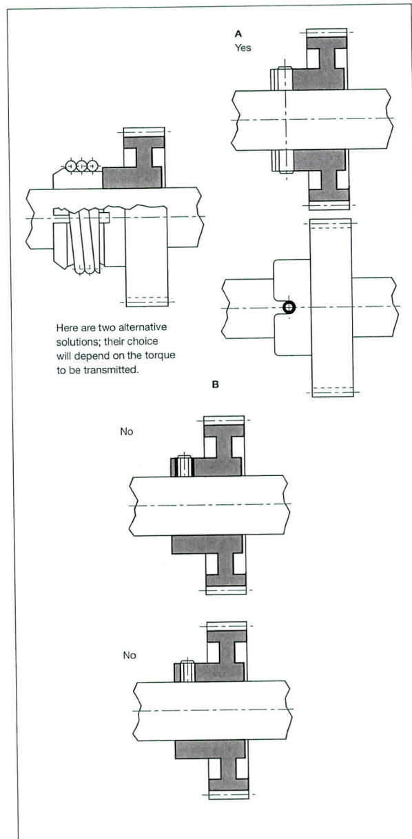
Fig. 8.19 Alternatives for grub screws
