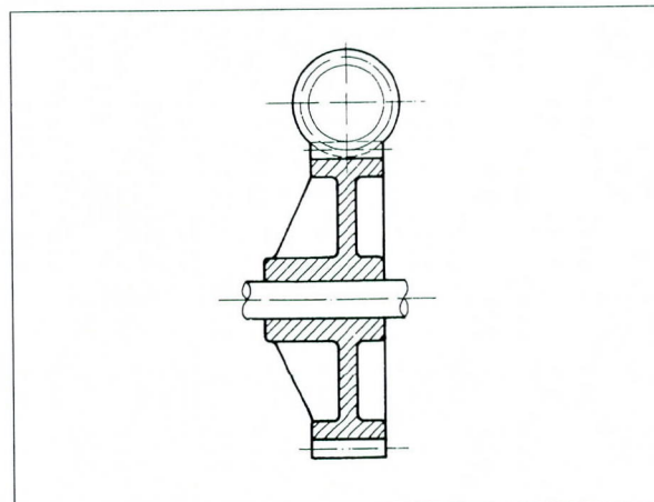
Fig. 8.07 Ribbed worm take-off gear
