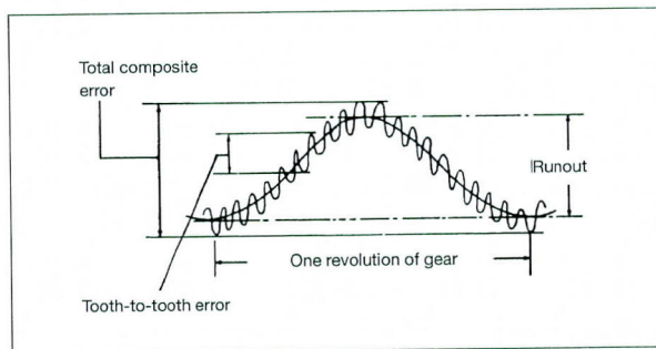
Fig. 8.11-c Center distance variation diagram
