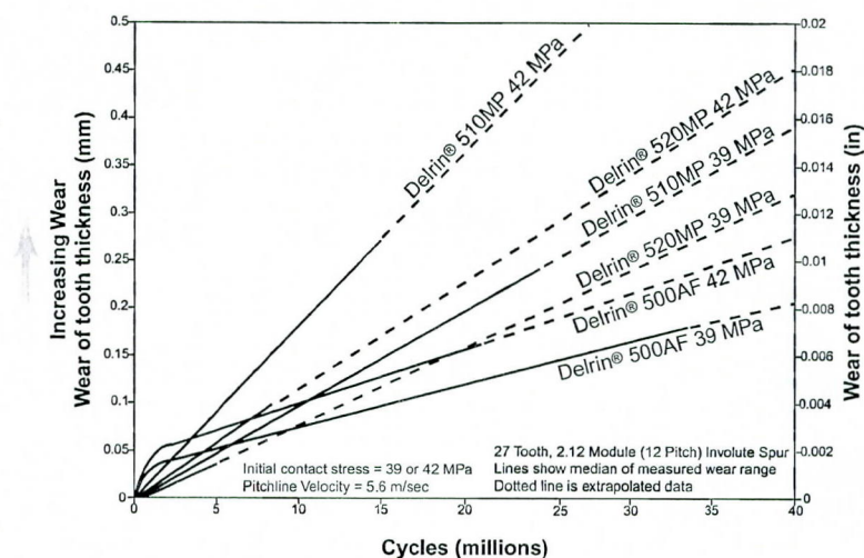
Figure 4. Sensitivity to Load—Delrin® Against Steel
