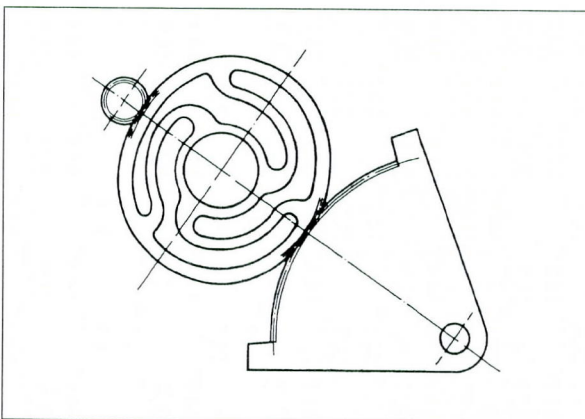
Fig. 8.22 Backlash-free gear
