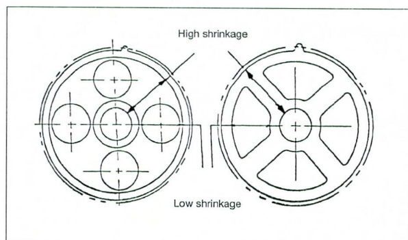
Fig. 8.08 Holes and ribs in moulded gears
