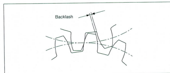
Fig. 8.11-e Measurement of backlash
