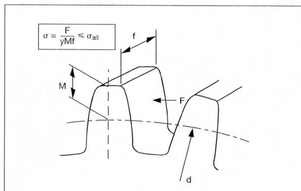
Fig. 8.02 Gear design
