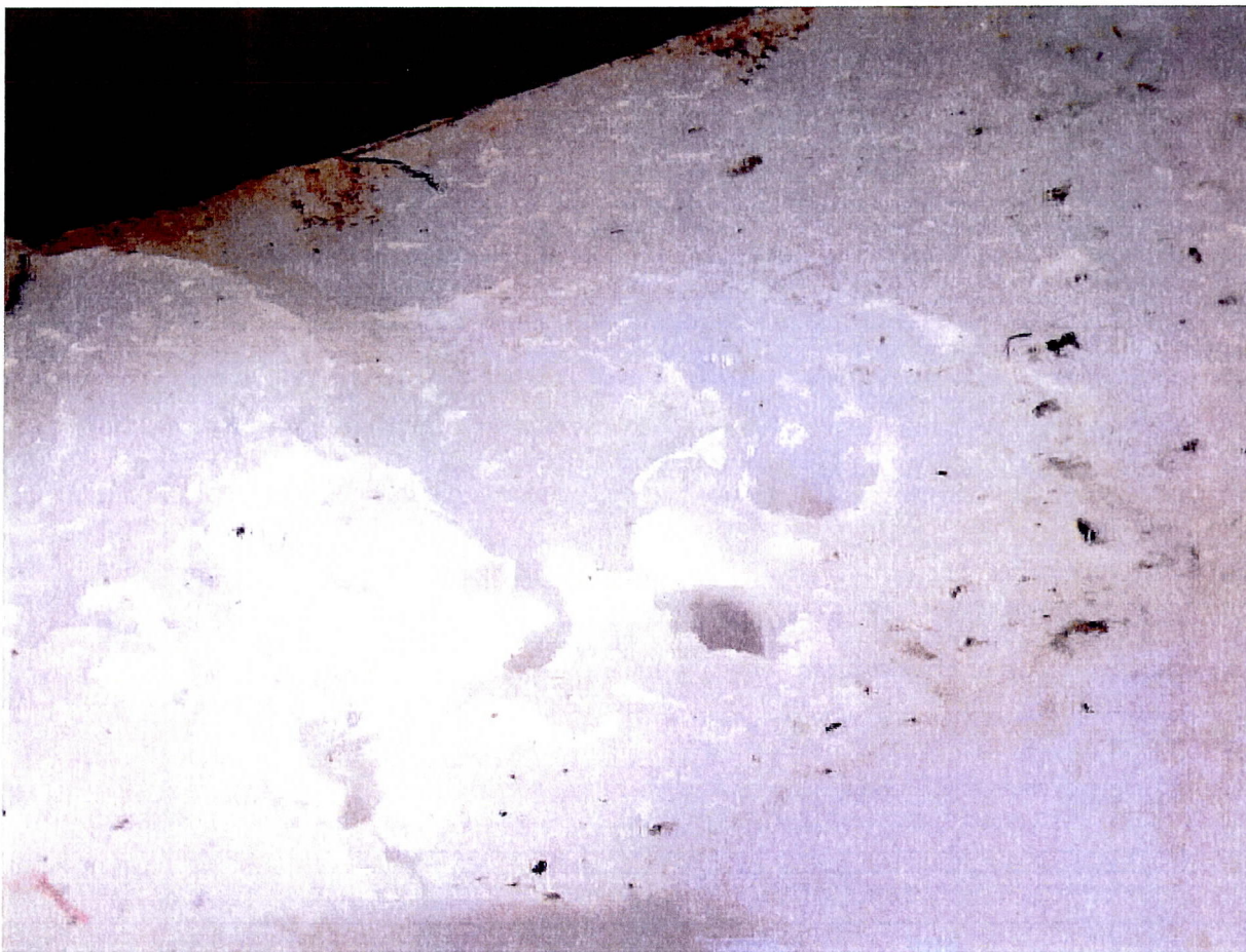
Voids in polymer, poor polymer flow/ weld.
