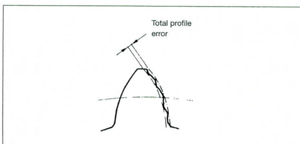
Fig. 8.11-a Measurement of tooth profile error
