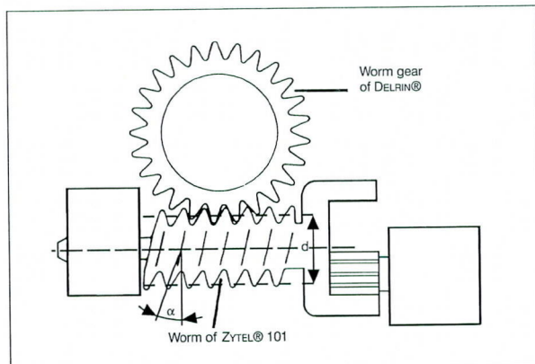
Fig. 8.18 Can opener with worm drive
