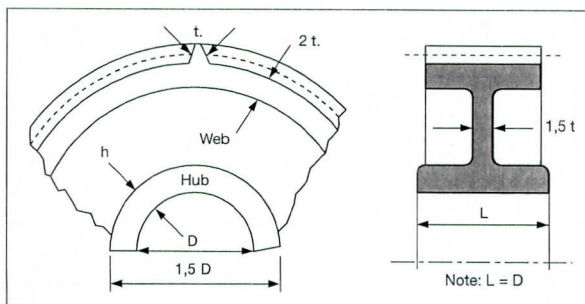
Fig. 8.03 Suggested gear proportions
