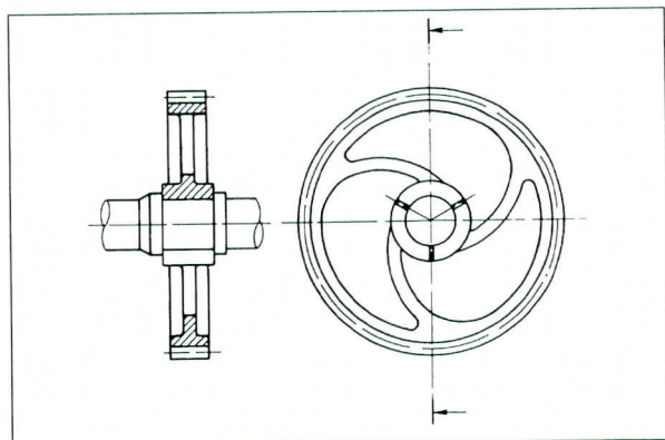
Fig. 8.25 Gear with sliding coupling
