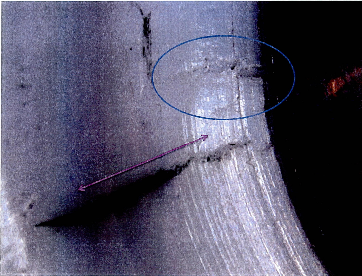
Radial fracture and stress lines at insert.
