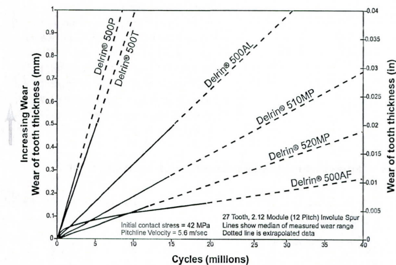
Figure 3. Unlubricated Wear of Gear Teeth—Delrin® Against Steel
