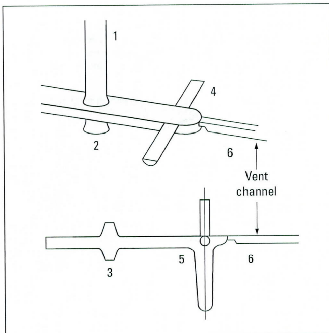
Figure 28. Key Rules for the Design of the Sprue and Runners of a 2 Plate Mold (Top) and of a 3 Plate Mold (Bottom).
