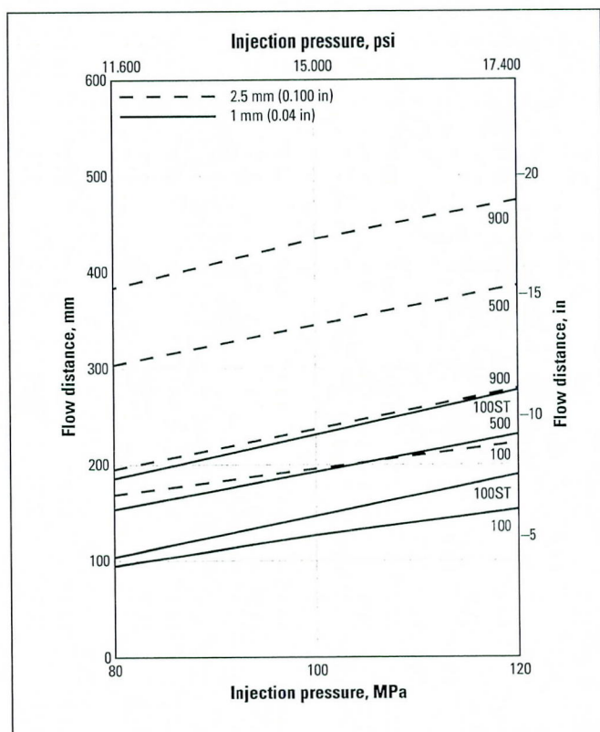
Figure 15. Maximum Flow Distance of Delrin® Acetal Resins
