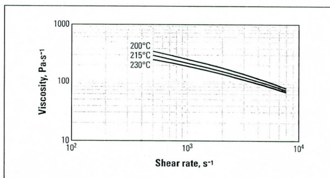
Figure 7. Viscosity versus Shear Rate of Delrin® 500P at Three Temperatures
