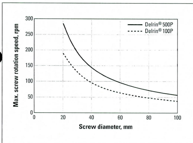
Figure 36. Maximum Screw Rotation Speed as Function of Screw Diameter. The Curve for Delrin® 500P is Also Valid for the Low Viscosity Grades Delrin® 900.
