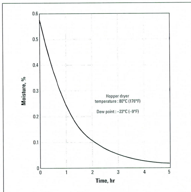
Figure 50. Drying Behavior of Delrin® 100ST
