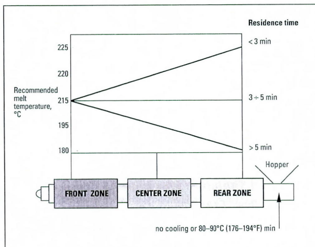
Figure 35. Cylinder Temperatures Profile Versus Residence Time for a Given Recommended Melt Temperature. Recommended Nozzle Temperature is 190°C (374°F) for All Delrin® Grades.
