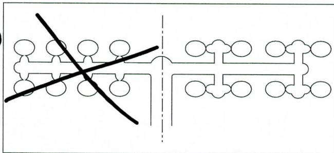
Figure 23. Examples of Unbalanced 16-Cavity Mold. The Solution on the Right is Provided with Overflow Wells to Trap Cold Slugs.
