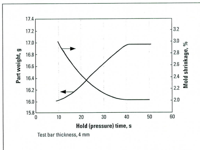
Figure 41. Hold (Pressure) Time Versus Part Weight and Mold Shrinkage of Delrin® 500P
