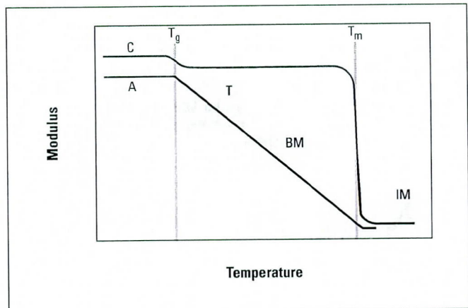
Figure 29. Softening/Melting Behaviour of Amorphous and Crystalline Polymers
