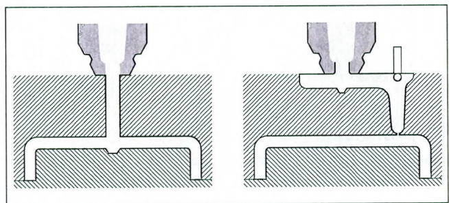
Figure 21. Direct Gating (Left) and Indirect Gating to Break the Flow (Right), in a One-Cavity Mold
