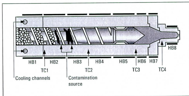
Figure 10. The Risk of Black Specks Contamination That Could Arise From the Presence of a Cooling System of the Feed Throat
