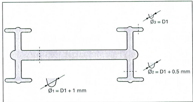
Figure 20. Correct Runner Thickness for an Eight Cavity Mold
