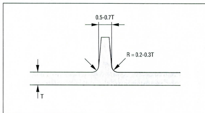
Figure 33. Suggested Rib Dimensions Versus Wall Thickness
