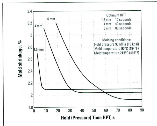
Figure 44. Effect of Hold (Pressure) Time on Mold Shrinkage of Delrin® 500P
