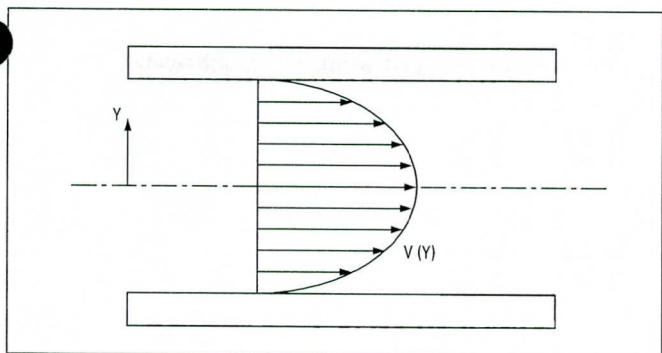
Figure 6. Approximate Shape of the Velocity Distribution Between Two Parallel Plates. The Shear Rate is the Derivative dv(y)/dy .
