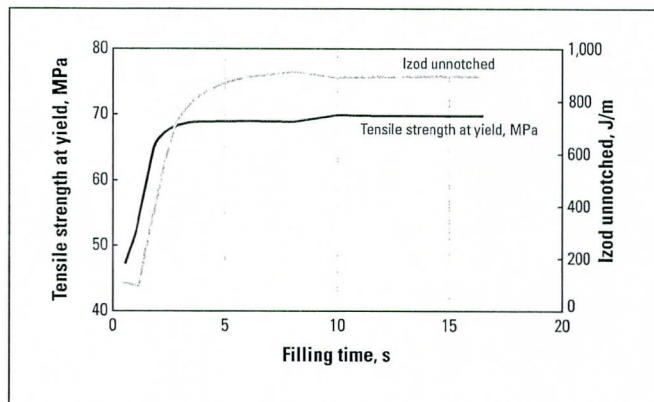
Figure 34. Tensile Strength (Left Scale) and Unnotched Izod Impact (Right Scale) of a Delrin® 100P Test Bar, 4 mm thick, Molded at Both Ends with Different Filling Times.
