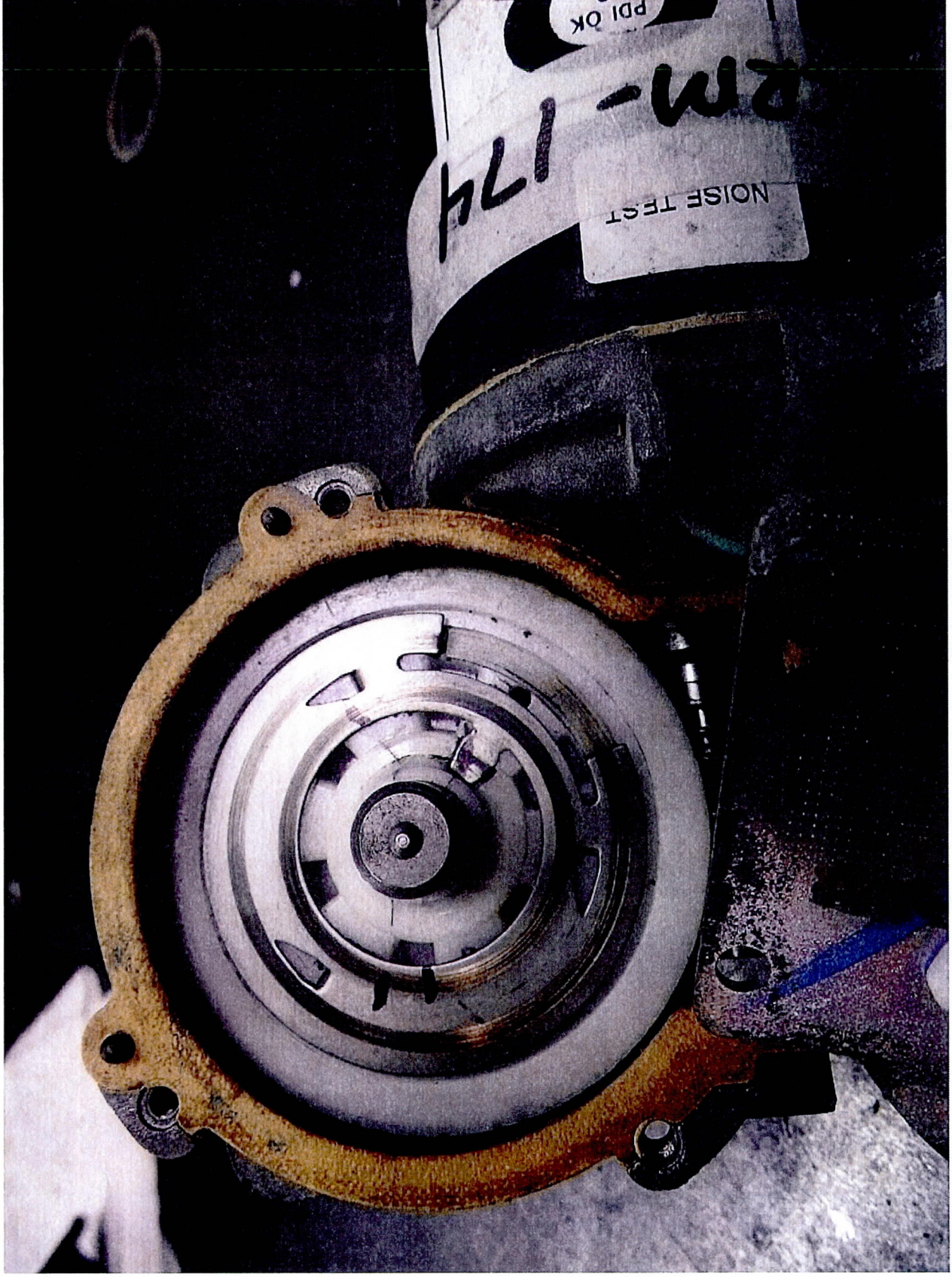
Gear with cracks starting at shaft (grease removed). 150,000 miles, 15.5 months in service.
