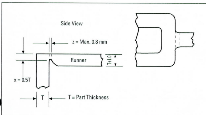
Figure 17. Details of a Typical Edge Gate Suitable for Delrin®
