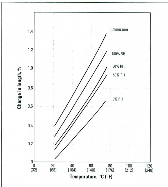
Figure 48. Environmental Dimensional Change of Delrin® 100 and 500
