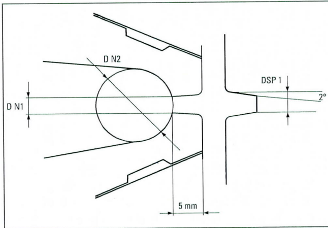
Figure 27. Example of a Design of a Nozzle without Sprue Used with 3 Plate Molds. Remember that for Delrin® the Nozzle Temperature Should Not Exceed 190°C (374°F).
