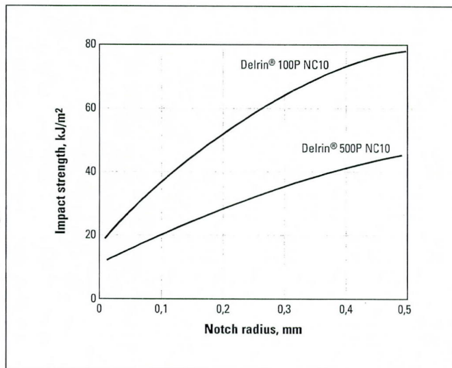
Figure 32. Impact Strength as a Function of Molded Notch Radius
