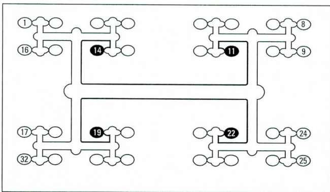
Figure 24. Example of "Spiral Effect" in a 32-Cavity Mold. Cavities 11, 14, 19, 22 Will Be Filled First and May Show Splays and Mold Deposits.
