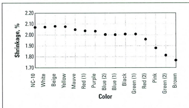
Figure 46. Effect of Selected Pigments on Mold Shrinkage of Delrin® 500P. Part Thickness 2 mm
