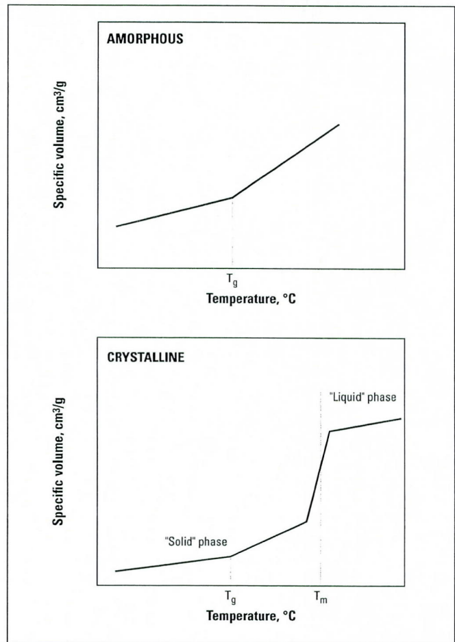
Figure 1. Specific Volume as Function of Temperature for Amorphous And Crystalline Polymers
