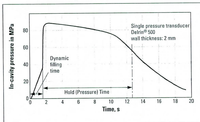
Figure 42. Cavity Pressure Measured During the Filling and Packing (1 sensor)
