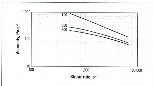
Figure 8. Viscosity versus Shear Rate for Various Grades of Delrin® at a Constant Temperature of 215°C (419°F)
