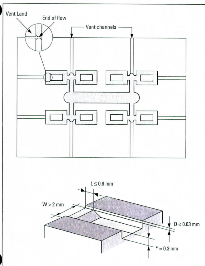
Figure 30. Recommended Venting of a Part and of its Runner System
