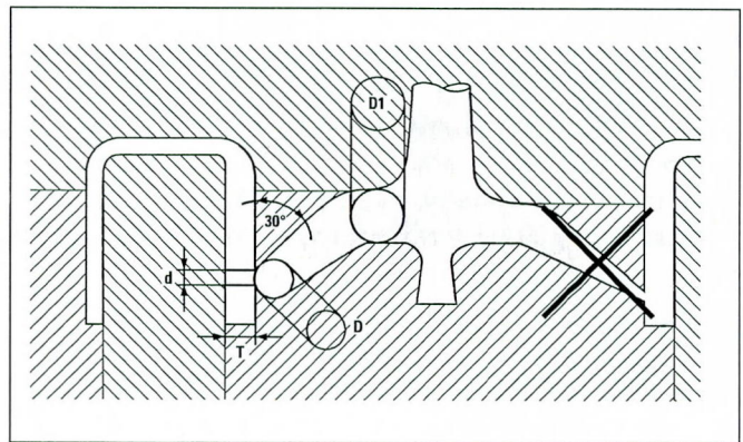
Figure 18. Details of a Submarine Gate (Tunnel Gate) Adequate for Delrin® (left side). The One on the Right is Not Adequate for Crystalline Polymers and Would Give Problems with Delrin®.
