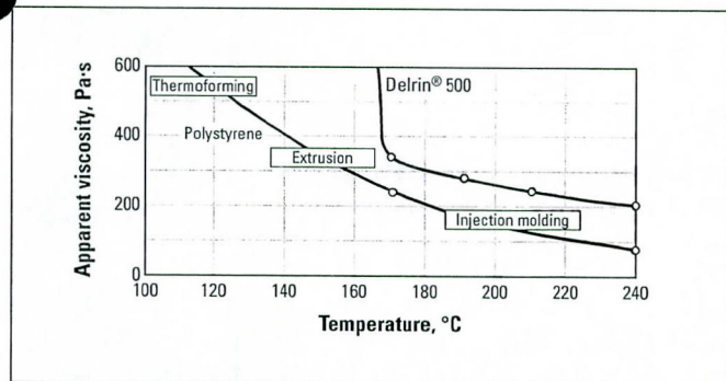
Figure 5. Viscosity/Temperature Curves for Delrin® 500P and for Polystyrene at a Constant Shear Rate of 1000 s -1 (Temperature Reduced from 230 to 100°C [446 to 212°F])
