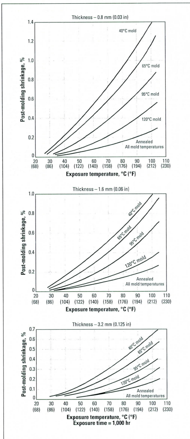
Figure 47. Post-Molding Shrinkage of Delrin® Acetal Resins
