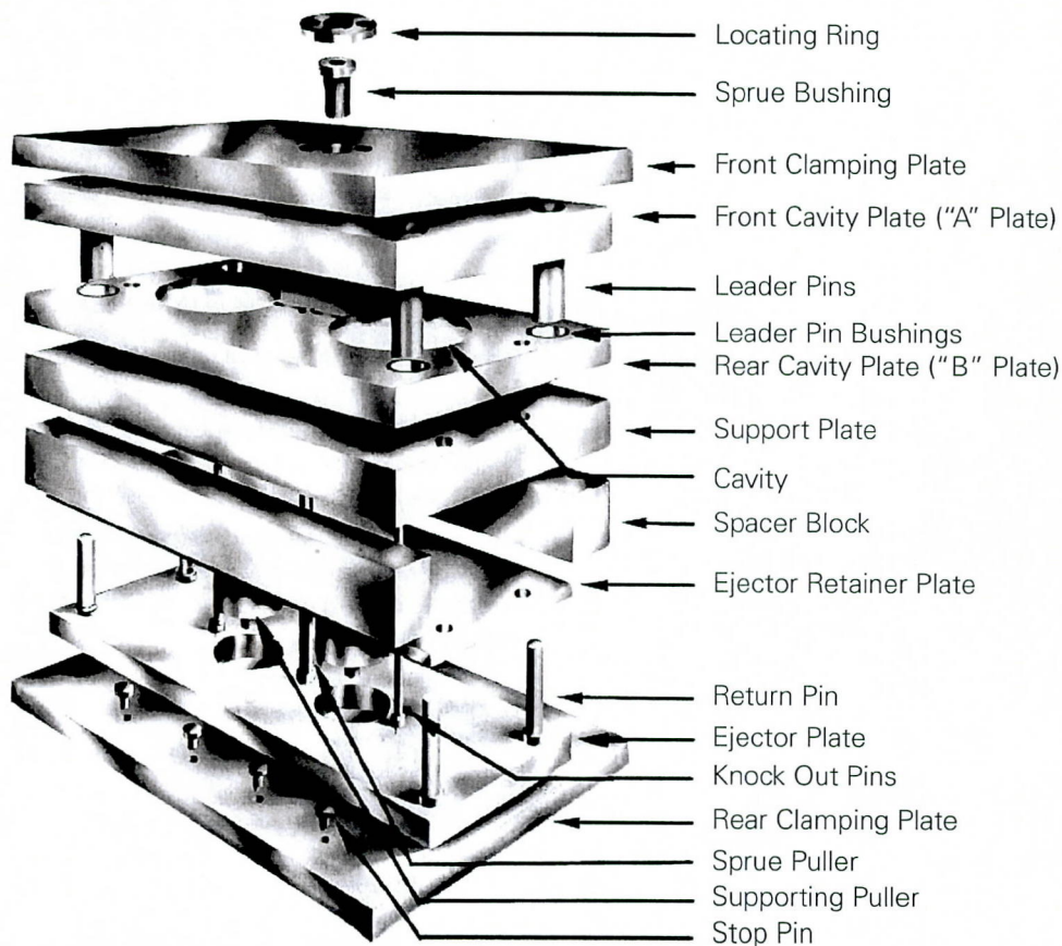
Figure 14. Exploded View of Mold
