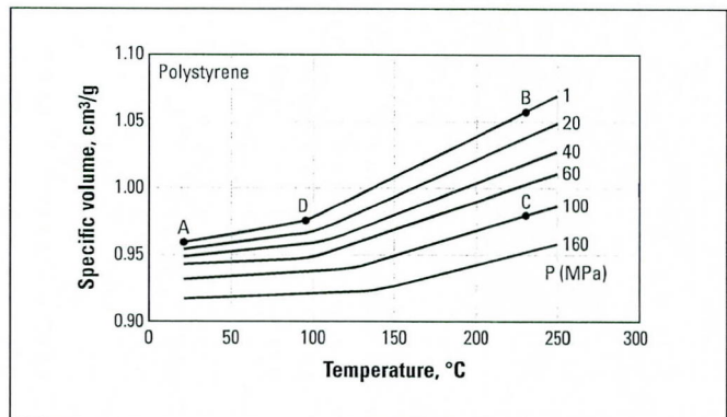
Figure 2. Pressure-Volume-Temperature (PVT) Diagram for Polystyrene. Points A, B, C, and D Refer to Different Steps of the Molding Process (see text).
