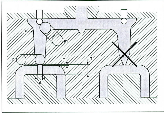
Figure 19. Details of a Three Plate Gate Design Adequate for Delrin® (Left Side). The One on the Right is Not Adequate for Crystalline Polymers and Would Give Problems with Delrin®. *Gate Length Should be <0.8 mm (0.03 in).
