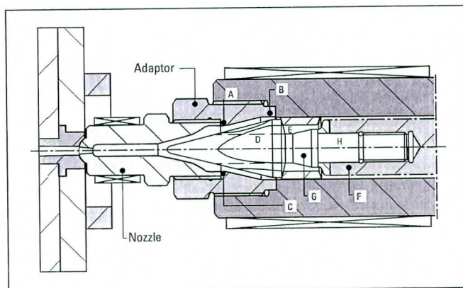
Figure 11. Design of Adaptor and Non-Return Valve
