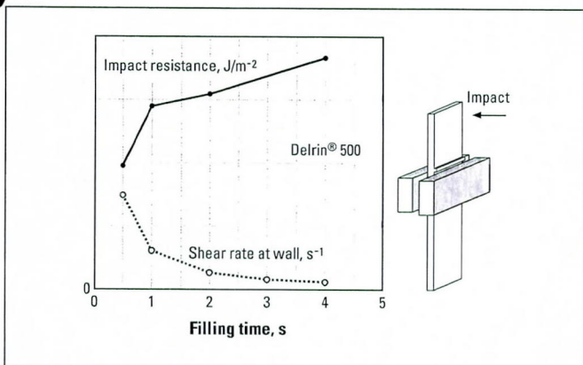
Figure 39. Shear Strain Rate at the Wall ( s^{-1} ) and Impact Resistance ( J/m^2 ) as Function of the Filling Time. This Data was Obtained with the Sample Shown (180 by 27 mm with 2 mm thickness). For Impact Resistance, the Part is Clamped Under the Rib and Hit by a Pendulum.
