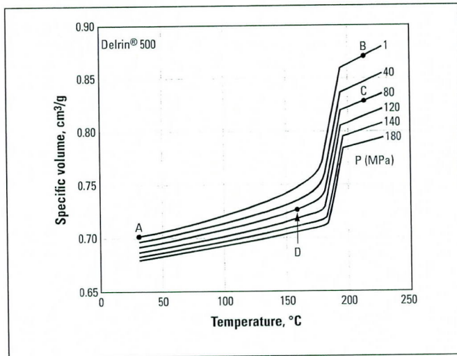
Figure 3. Pressure-Volume-Temperature (PVT) Diagram For Delrin® 500. Points A, B, C, and D Refer to Different Steps of the Molding Process (see text).
