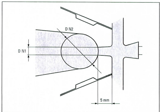
Figure 26. Example of a Design of a Nozzle Without Sprue Used with 2 Plate Molds. Remember that for Delrin® the Nozzle Temperature Should Not Exceed 190°C (374°F).
