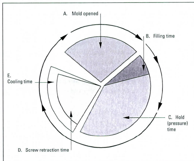
Figure 37. The Molding Cycle for Delrin®
