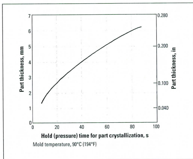
Figure 40. Hold (Pressure) Time Versus Part Thickness of Delrin® 500P
