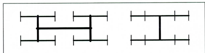
Figure 22. Balanced (Left) and Unbalanced (Right) Runner Systems in a 16-Cavity Mold
