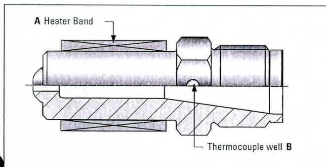
Figure 12. Reverse Taper Nozzle
