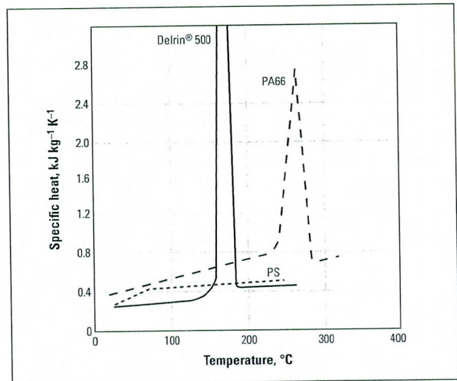
Figure 4. Specific Heat versus Temperature for Delrin® 500, PA66 and Polystyrene
