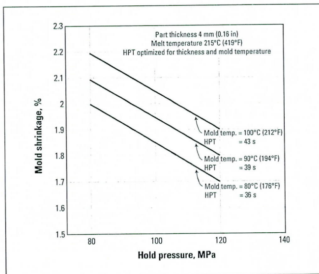
Figure 43. Effect of Hold Pressure on Mold Shrinkage at Three Mold Temperatures, for Delrin® 500P. Hold Pressure Can be Used for Small Adjustments of Part Dimensions, as it has Negligible Effect on Post-Molding Shrinkage.
