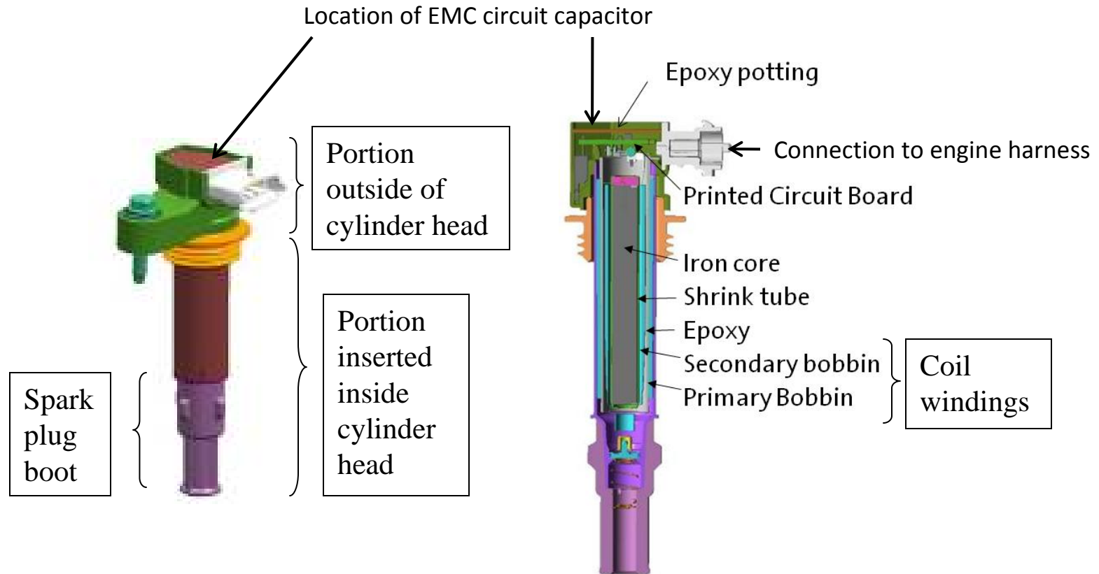
Anatomy of a Modern Automotive Ignition Coil (typical of those used in Saab 9.3)
