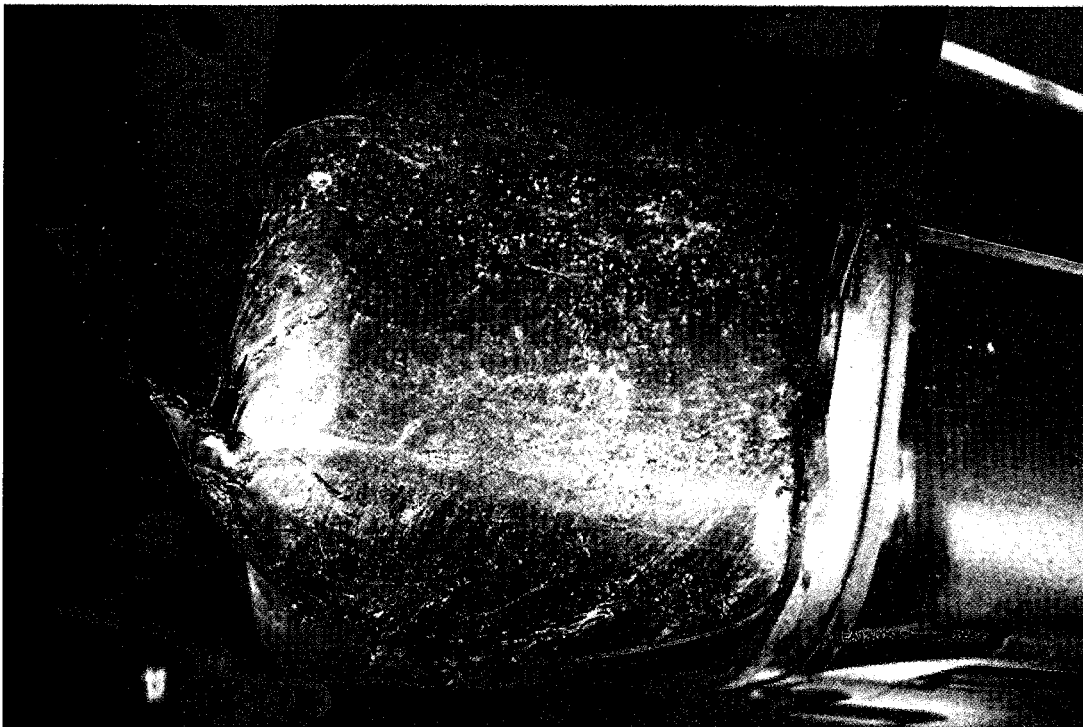
Figure 4 Rear Impact Damaged 2002 Liberty Fuel Tank.
