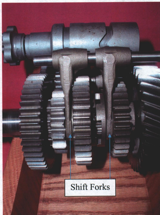
Figure 7 – Shift Forks and Drum
