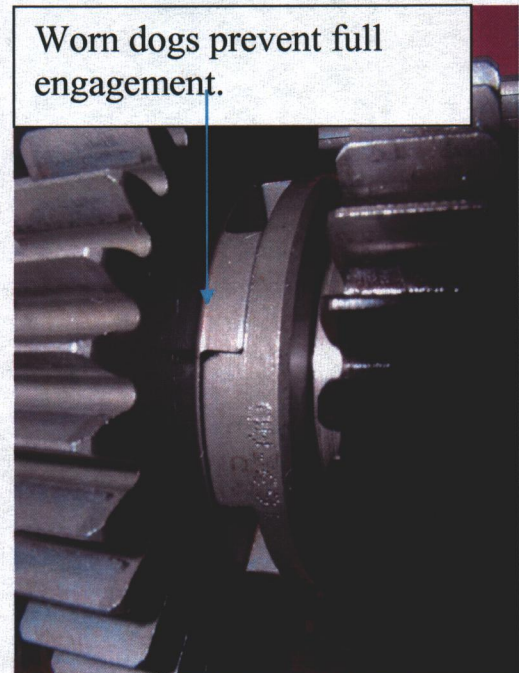
Figure 11 – Worn Engagement Dogs – 13,153 miles
