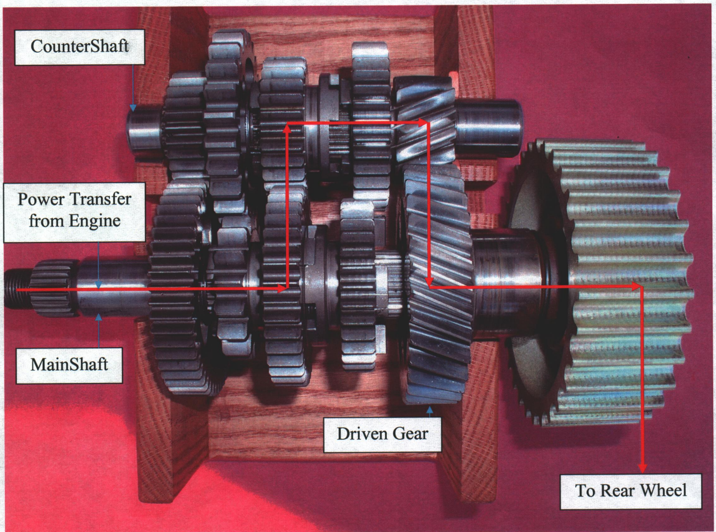
Figure 2. Gearsets and Power transfer
