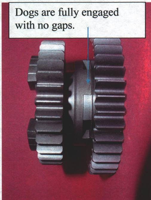
Figure 10 – Engagement Dogs – New
