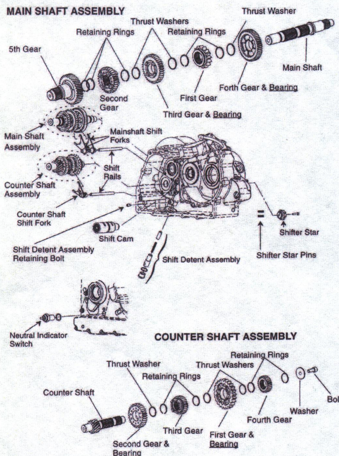
Figure 1. Subject Vehicle Internal Transmission Components, 1999 V92C Service Manual
