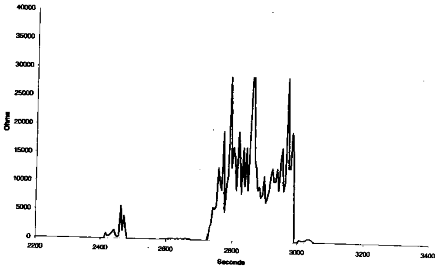
Terminal Resistance vs. Time 5% Salt Water Ingress Experiment
