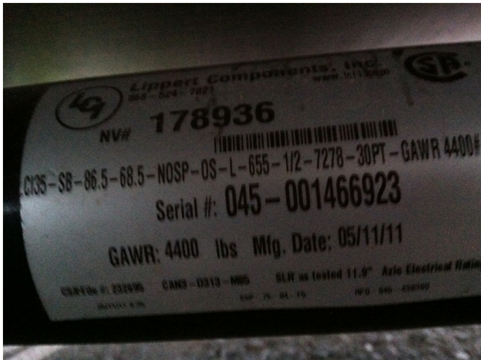
Rear Axle Label
